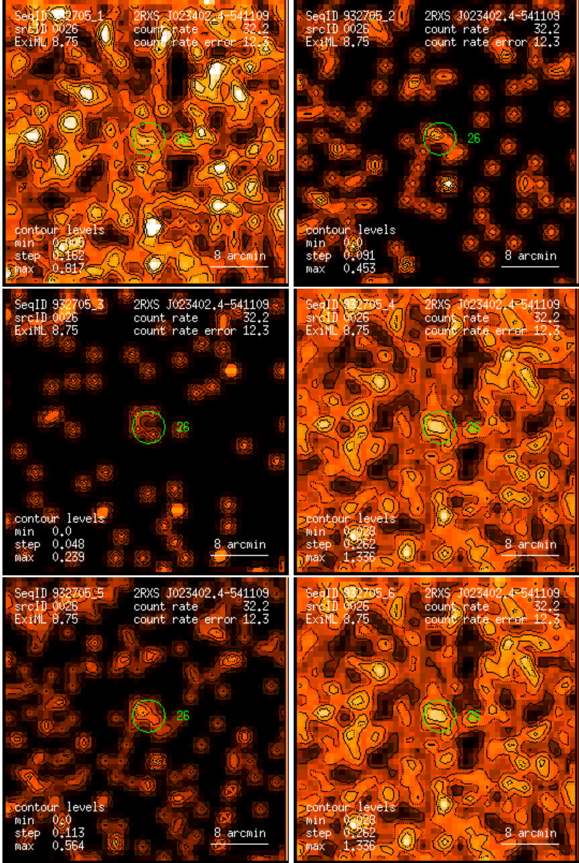
Figure 26: RASS 932705: detection 0026: band rate images, Gaussian filter: (1) PSPC channels 11 – 41, (2) 52 – 90, (3) 91 – 201, (4) 11 – 235, (5) 52 – 201, (6) 11 – 201. Broad band rates in counts/ks. Band rate contour levels in counts/ks/arcmin 2 .
