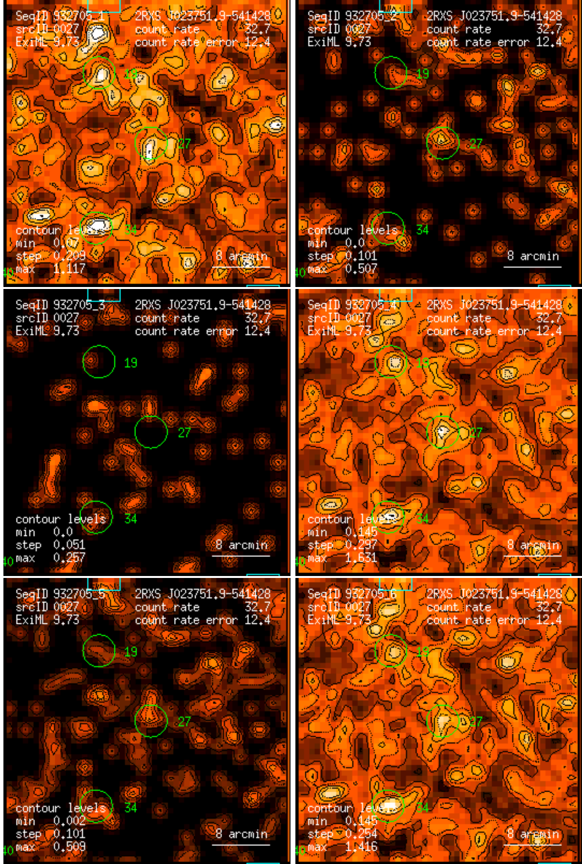
Figure 27: RASS 932705: detection 0027: band rate images, Gaussian filter: (1) PSPC channels 11 – 41, (2) 52 – 90, (3) 91 – 201, (4) 11 – 235, (5) 52 – 201, (6) 11 – 201. Broad band rates in counts/ks. Band rate contour levels in counts/ks/arcmin 2 .
