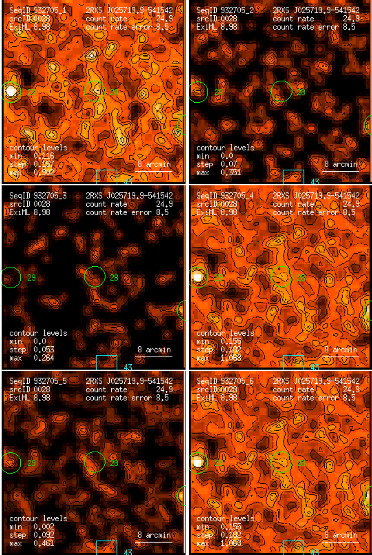
Figure 28: RASS 932705: detection 0028: band rate images, Gaussian filter: (1) PSPC channels 11 – 41, (2) 52 – 90, (3) 91 – 201, (4) 11 – 235, (5) 52 – 201, (6) 11 – 201. Broad band rates in counts/ks. Band rate contour levels in counts/ks/arcmin 2 .
