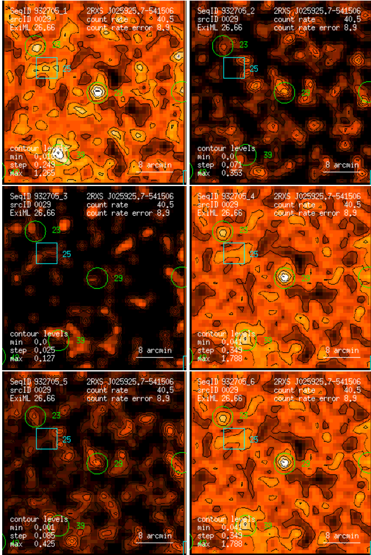
Figure 29: RASS 932705: detection 0029: band rate images, Gaussian filter: (1) PSPC channels 11 – 41, (2) 52 – 90, (3) 91 – 201, (4) 11 – 235, (5) 52 – 201, (6) 11 – 201. Broad band rates in counts/ks. Band rate contour levels in counts/ks/arcmin 2 .
