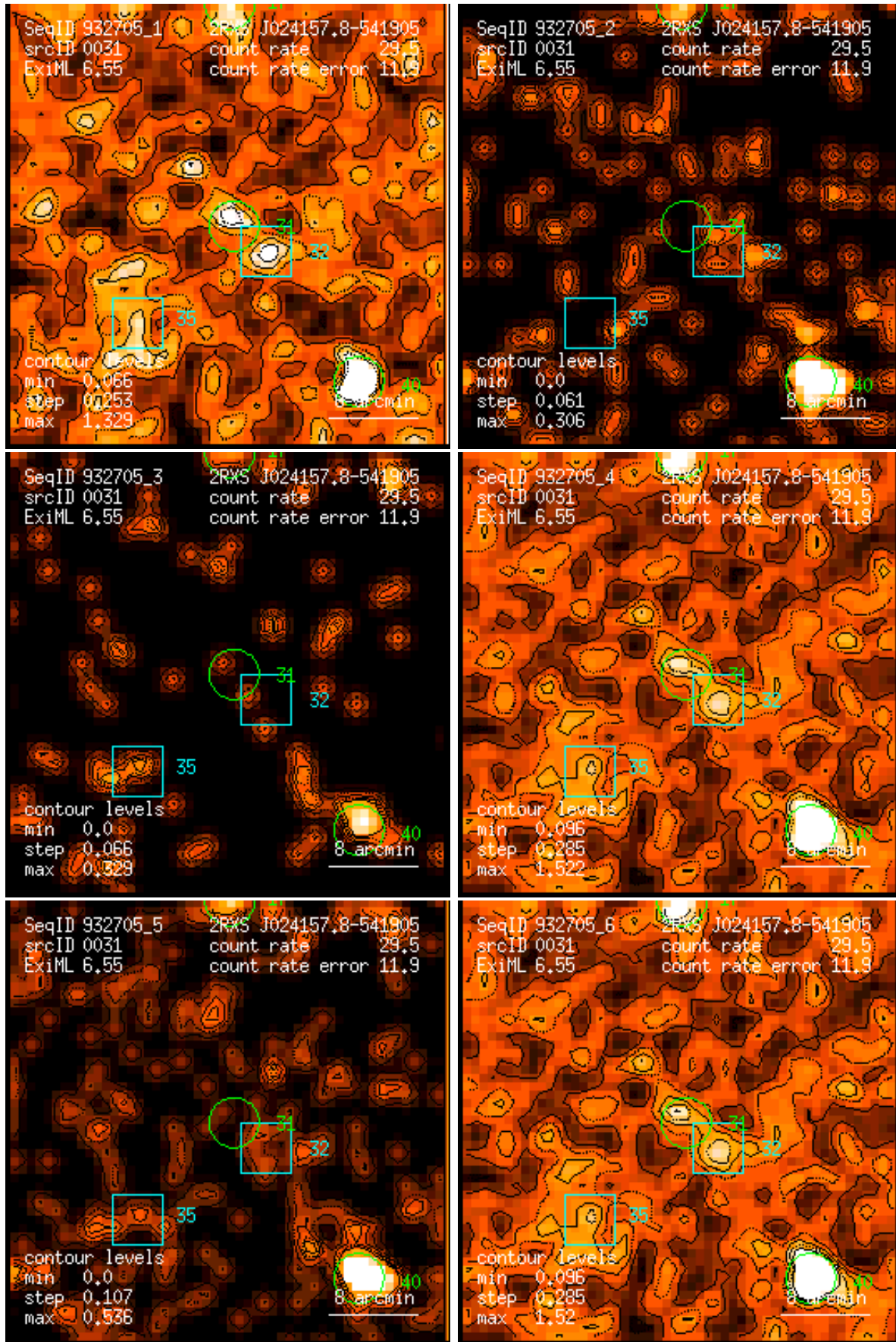
Figure 31: RASS 932705: detection 0031: band rate images, Gaussian filter: (1) PSPC channels 11 – 41, (2) 52 – 90, (3) 91 – 201, (4) 11 – 235, (5) 52 – 201, (6) 11 – 201. Broad band rates in counts/ks. Band rate contour levels in counts/ks/arcmin 2 .
