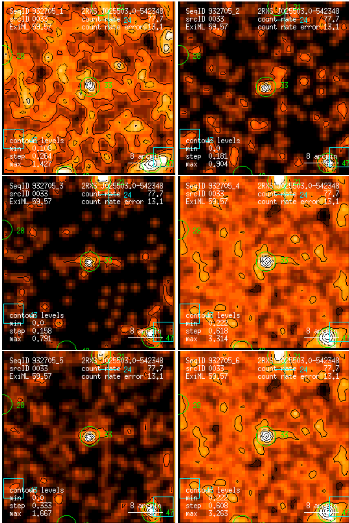
Figure 33: RASS 932705: detection 0033: band rate images, Gaussian filter: (1) PSPC channels 11 – 41, (2) 52 – 90, (3) 91 – 201, (4) 11 – 235, (5) 52 – 201, (6) 11 – 201. Broad band rates in counts/ks. Band rate contour levels in counts/ks/arcmin 2 .
