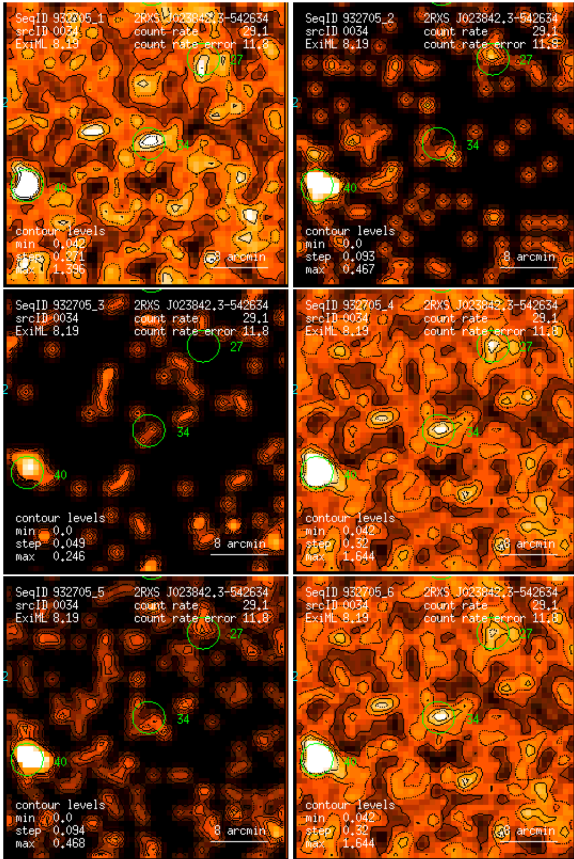
Figure 34: RASS 932705: detection 0034: band rate images, Gaussian filter: (1) PSPC channels 11 – 41, (2) 52 – 90, (3) 91 – 201, (4) 11 – 235, (5) 52 – 201, (6) 11 – 201. Broad band rates in counts/ks. Band rate contour levels in counts/ks/arcmin 2 .
