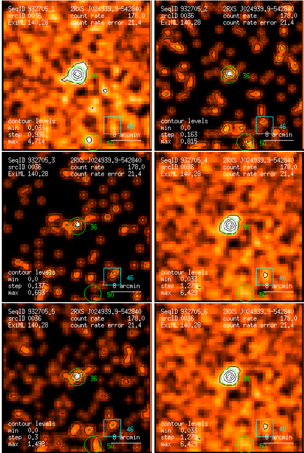
Figure 36: RASS 932705: detection 0036: band rate images, Gaussian filter: (1) PSPC channels 11 – 41, (2) 52 – 90, (3) 91 – 201, (4) 11 – 235, (5) 52 – 201, (6) 11 – 201. Broad band rates in counts/ks. Band rate contour levels in counts/ks/arcmin 2 .
