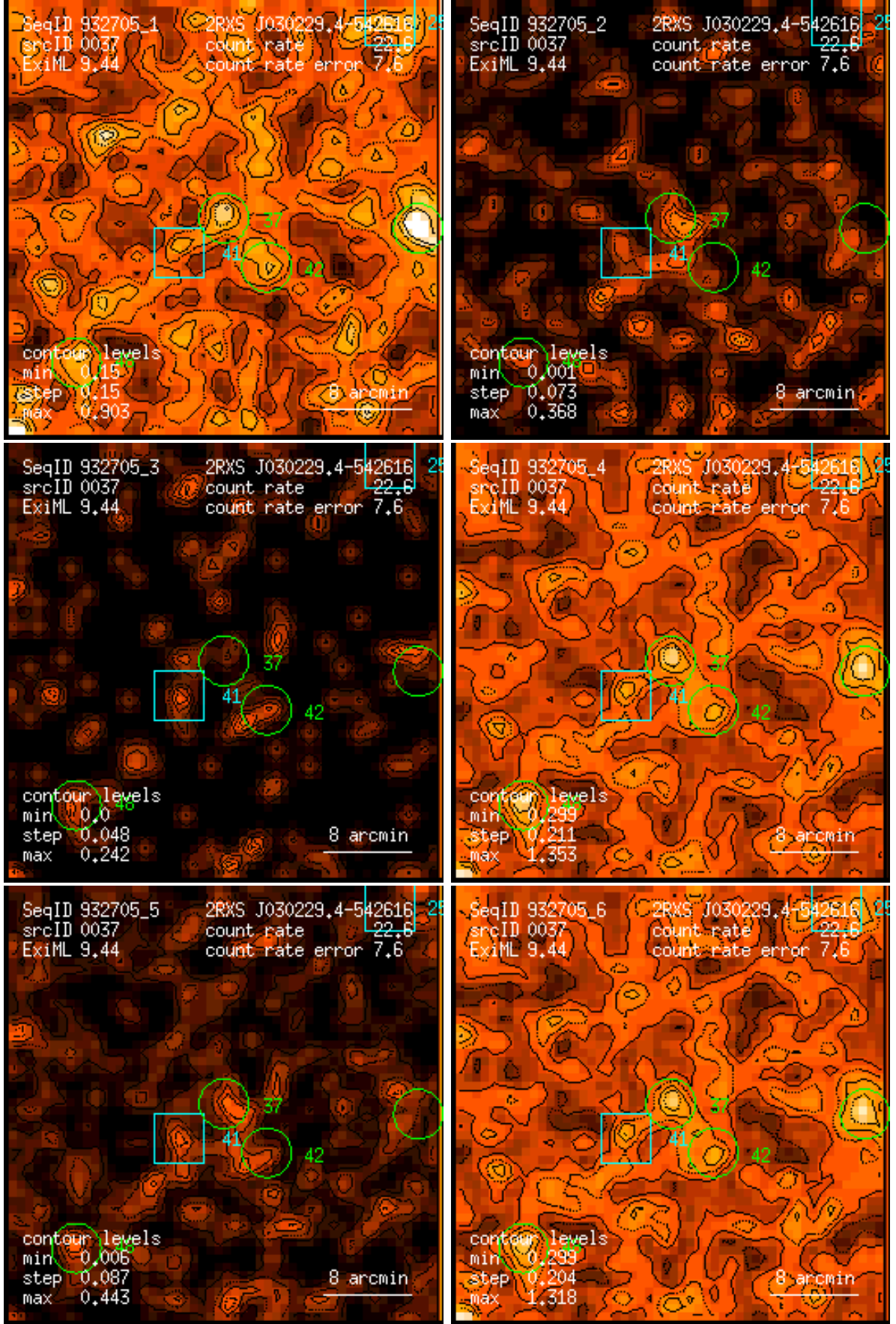
Figure 37: RASS 932705: detection 0037: band rate images, Gaussian filter: (1) PSPC channels 11 – 41, (2) 52 – 90, (3) 91 – 201, (4) 11 – 235, (5) 52 – 201, (6) 11 – 201. Broad band rates in counts/ks. Band rate contour levels in counts/ks/arcmin 2 .
