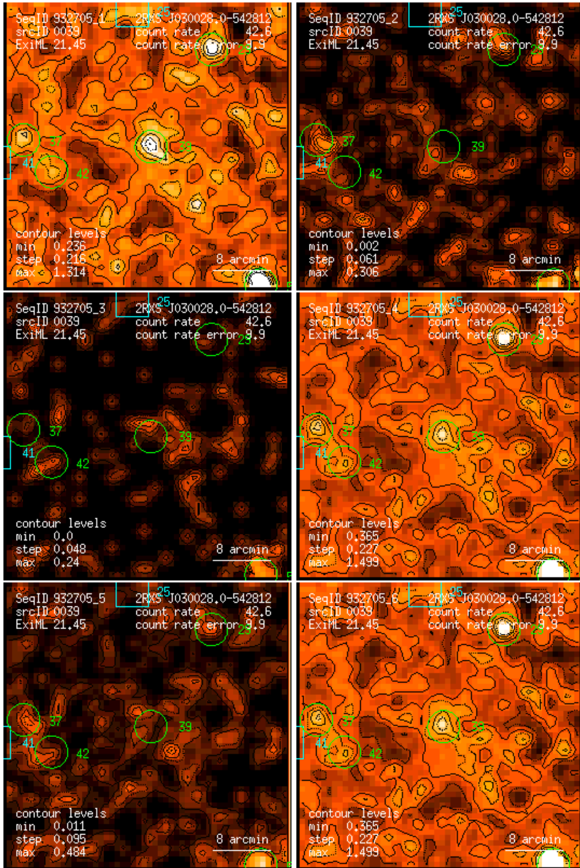
Figure 39: RASS 932705: detection 0039: band rate images, Gaussian filter: (1) PSPC channels 11 – 41, (2) 52 – 90, (3) 91 – 201, (4) 11 – 235, (5) 52 – 201, (6) 11 – 201. Broad band rates in counts/ks. Band rate contour levels in counts/ks/arcmin 2 .
