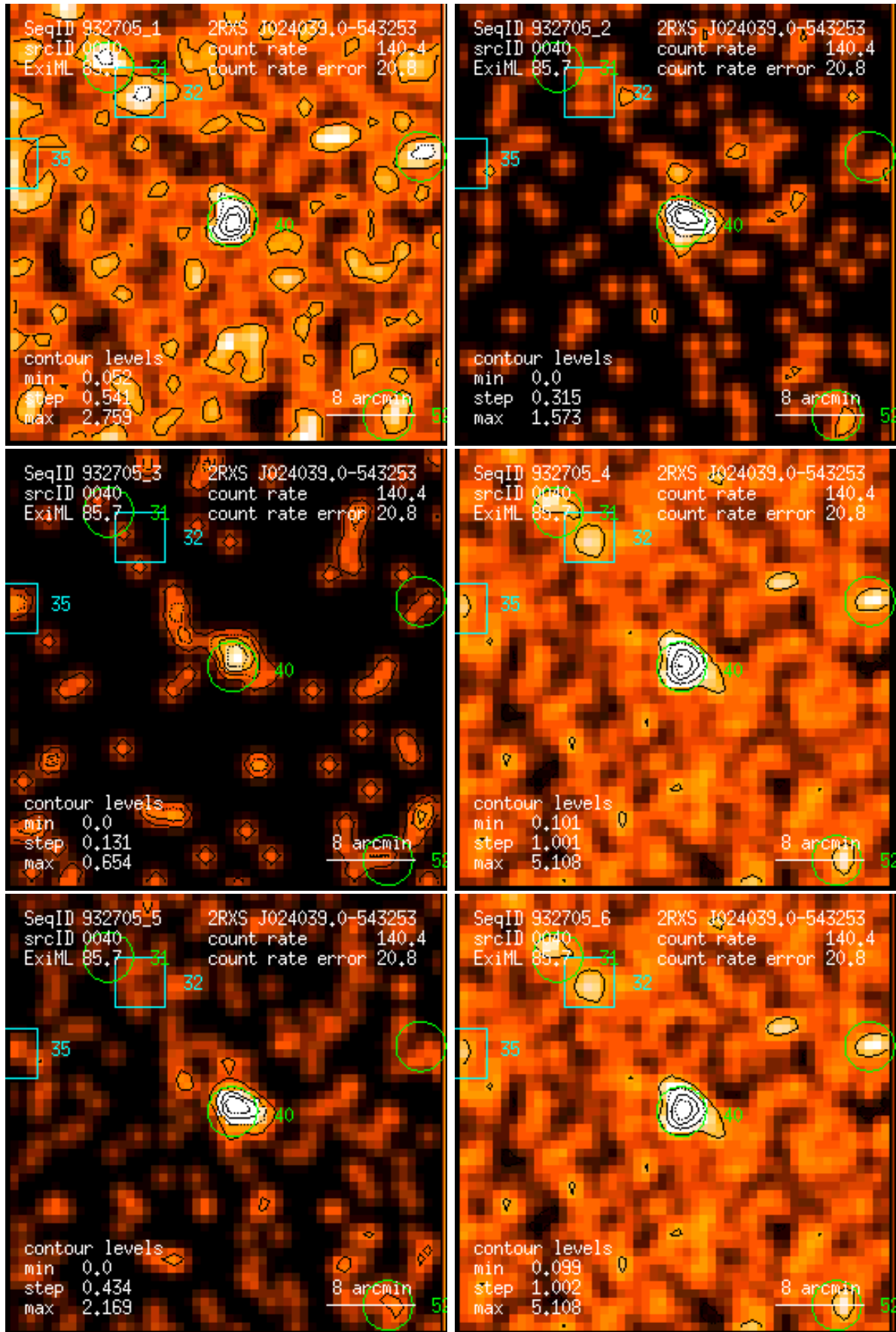
Figure 40: RASS 932705: detection 0040: band rate images, Gaussian filter: (1) PSPC channels 11 – 41, (2) 52 – 90, (3) 91 – 201, (4) 11 – 235, (5) 52 – 201, (6) 11 – 201. Broad band rates in counts/ks. Band rate contour levels in counts/ks/arcmin 2 .
