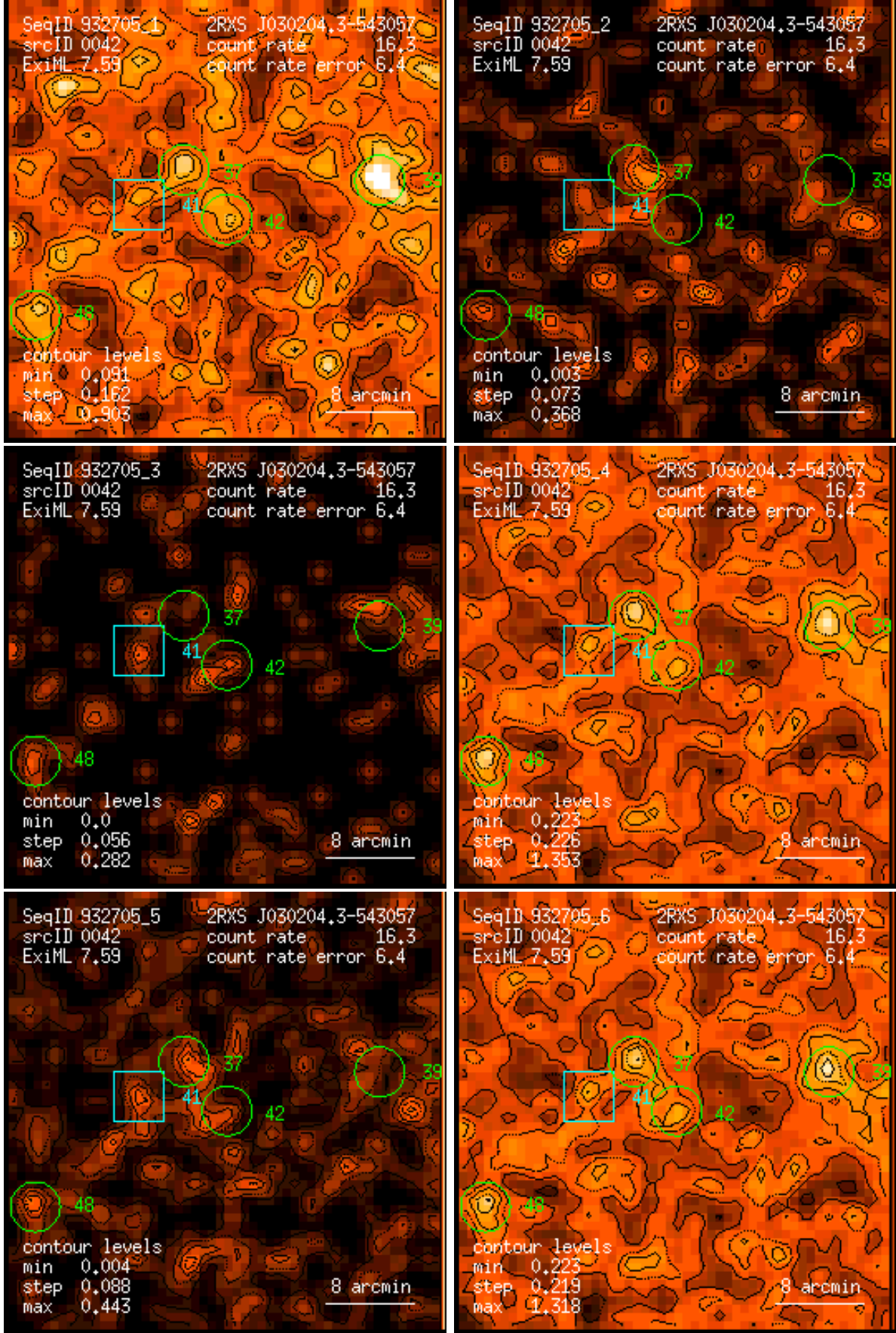
Figure 42: RASS 932705: detection 0042: band rate images, Gaussian filter: (1) PSPC channels 11 – 41, (2) 52 – 90, (3) 91 – 201, (4) 11 – 235, (5) 52 – 201, (6) 11 – 201. Broad band rates in counts/ks. Band rate contour levels in counts/ks/arcmin 2 .
