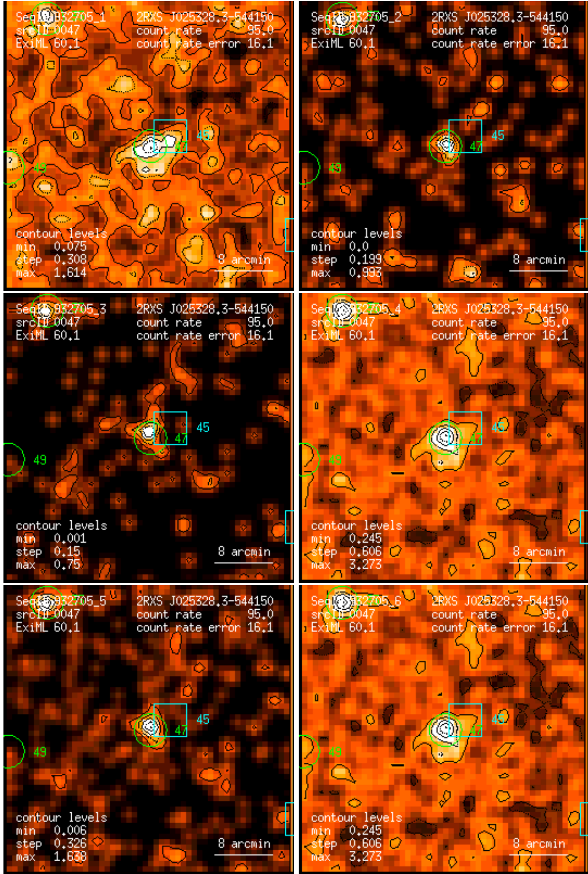
Figure 47: RASS 932705: detection 0047: band rate images, Gaussian filter: (1) PSPC channels 11 – 41, (2) 52 – 90, (3) 91 – 201, (4) 11 – 235, (5) 52 – 201, (6) 11 – 201. Broad band rates in counts/ks. Band rate contour levels in counts/ks/arcmin 2 .
