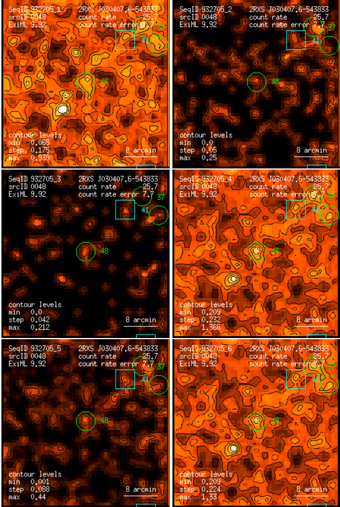
Figure 48: RASS 932705: detection 0048: band rate images, Gaussian filter: (1) PSPC channels 11 – 41, (2) 52 – 90, (3) 91 – 201, (4) 11 – 235, (5) 52 – 201, (6) 11 – 201. Broad band rates in counts/ks. Band rate contour levels in counts/ks/arcmin 2 .
