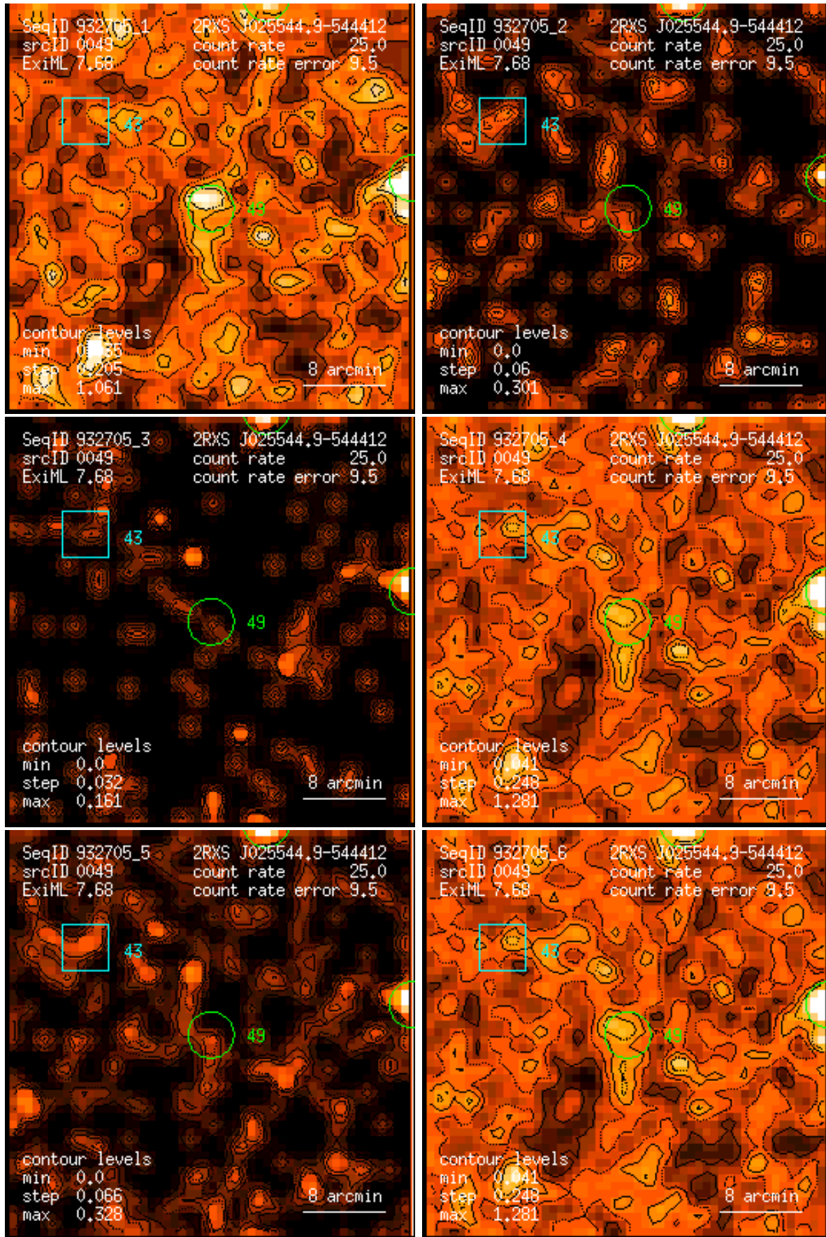
Figure 49: RASS 932705: detection 0049: band rate images, Gaussian filter: (1) PSPC channels 11 – 41, (2) 52 – 90, (3) 91 – 201, (4) 11 – 235, (5) 52 – 201, (6) 11 – 201. Broad band rates in counts/ks. Band rate contour levels in counts/ks/arcmin 2 .
