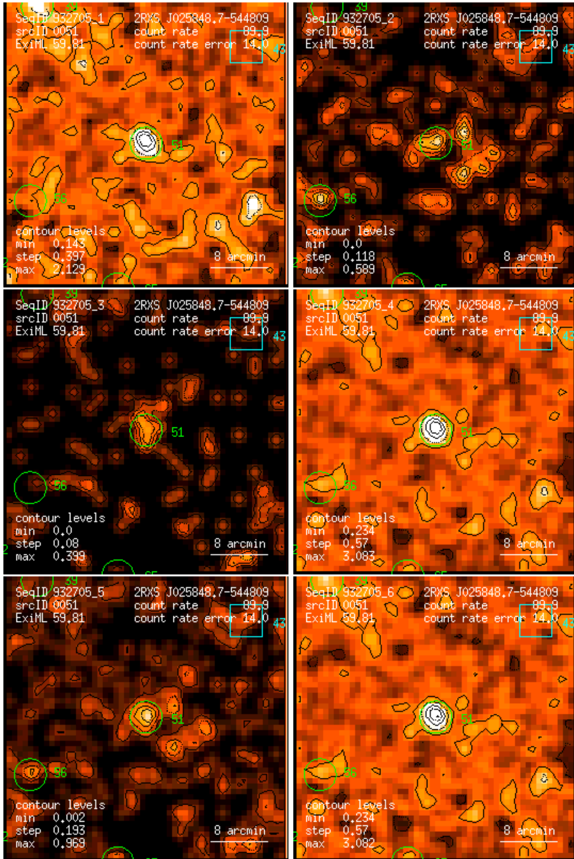
Figure 51: RASS 932705: detection 0051: band rate images, Gaussian filter: (1) PSPC channels 11 – 41, (2) 52 – 90, (3) 91 – 201, (4) 11 – 235, (5) 52 – 201, (6) 11 – 201. Broad band rates in counts/ks. Band rate contour levels in counts/ks/arcmin 2 .
