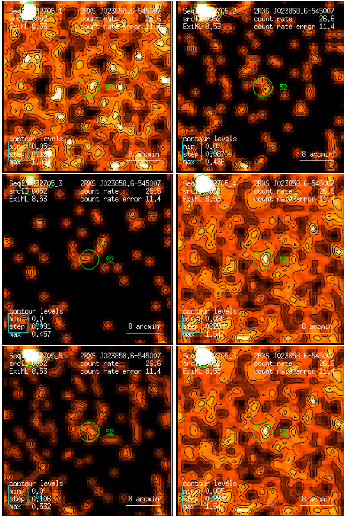
Figure 52: RASS 932705: detection 0052: band rate images, Gaussian filter: (1) PSPC channels 11 – 41, (2) 52 – 90, (3) 91 – 201, (4) 11 – 235, (5) 52 – 201, (6) 11 – 201. Broad band rates in counts/ks. Band rate contour levels in counts/ks/arcmin 2 .
