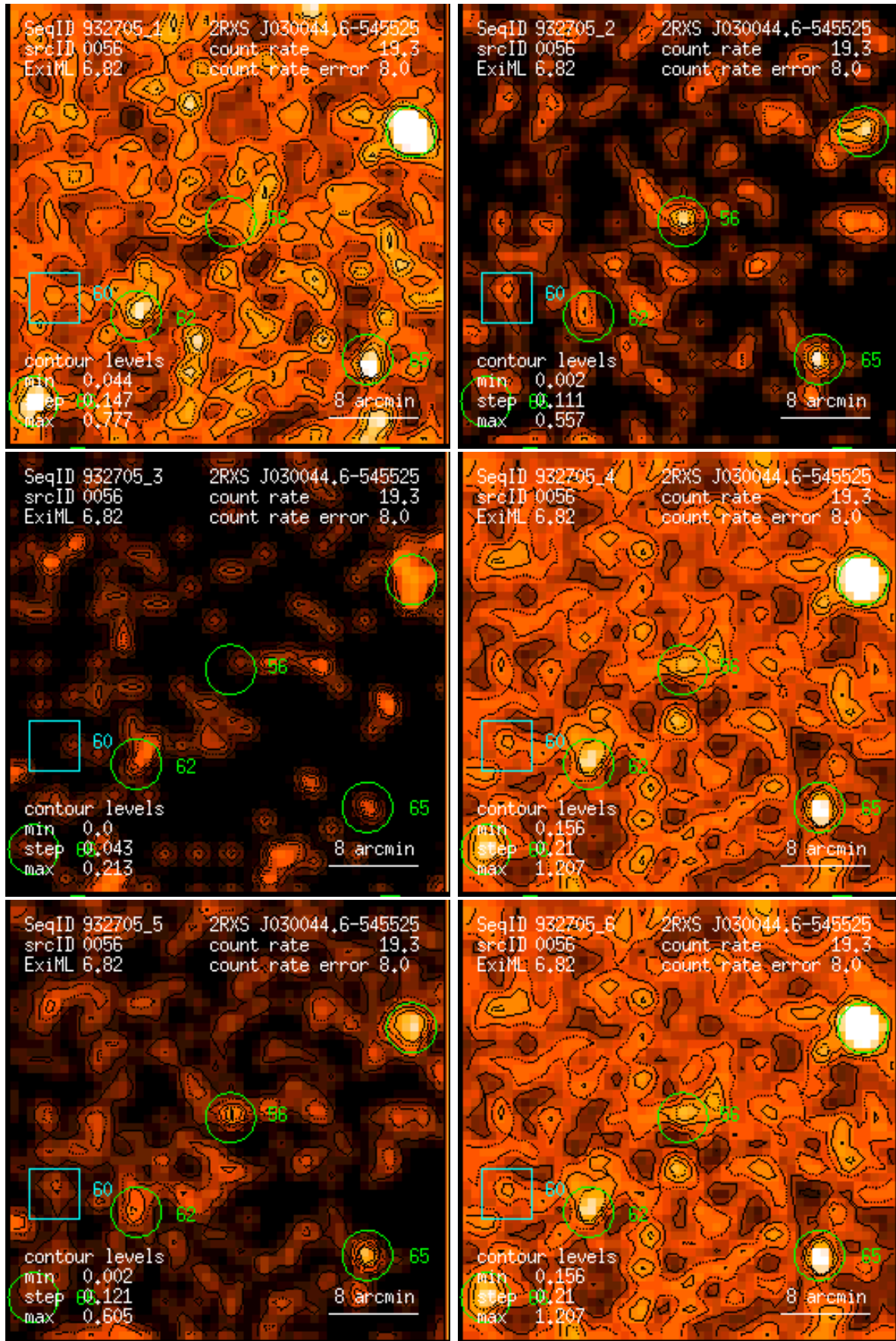
Figure 56: RASS 932705: detection 0056: band rate images, Gaussian filter: (1) PSPC channels 11 – 41, (2) 52 – 90, (3) 91 – 201, (4) 11 – 235, (5) 52 – 201, (6) 11 – 201. Broad band rates in counts/ks. Band rate contour levels in counts/ks/arcmin 2 .
