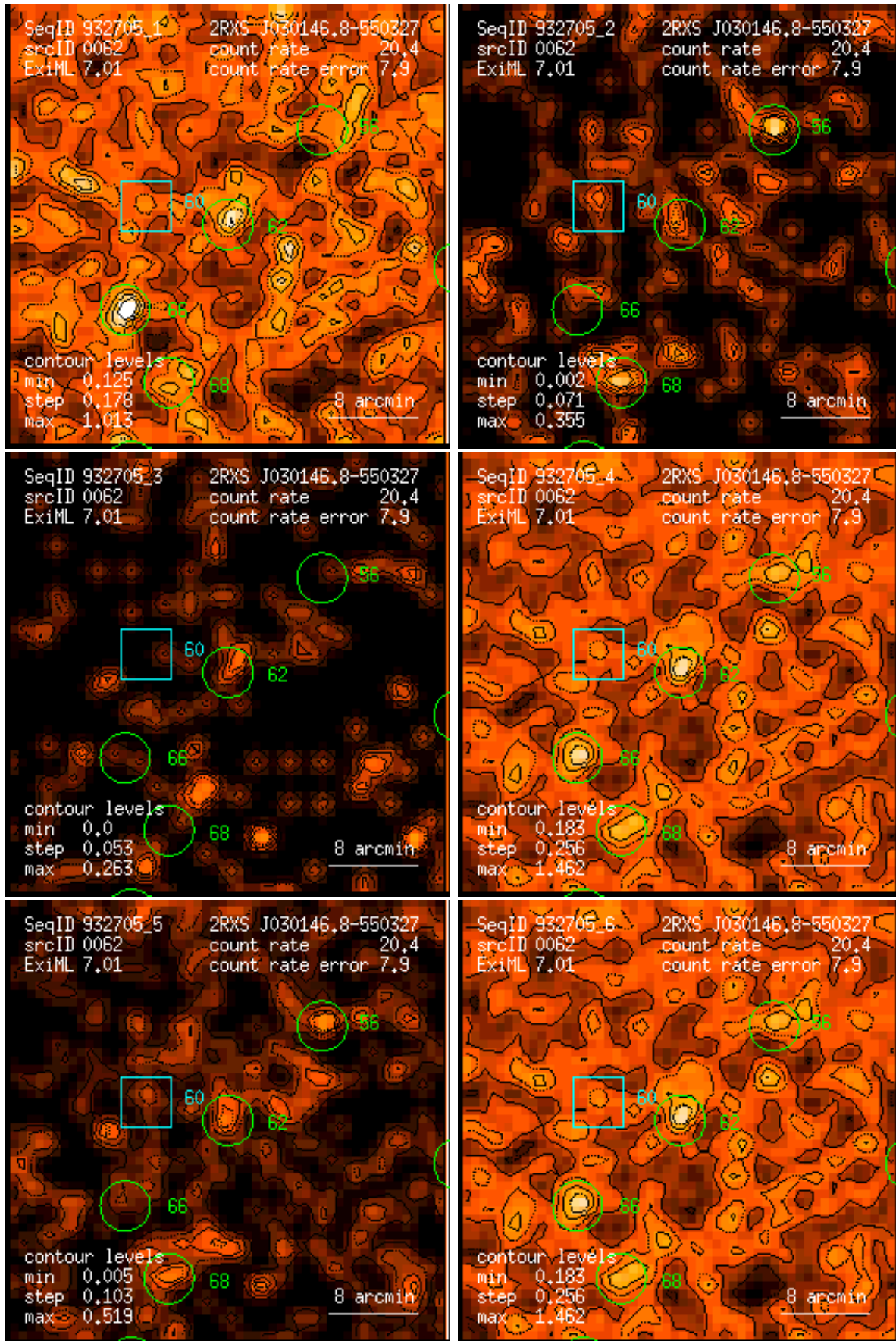
Figure 62: RASS 932705: detection 0062: band rate images, Gaussian filter: (1) PSPC channels 11 – 41, (2) 52 – 90, (3) 91 – 201, (4) 11 – 235, (5) 52 – 201, (6) 11 – 201. Broad band rates in counts/ks. Band rate contour levels in counts/ks/arcmin 2 .
