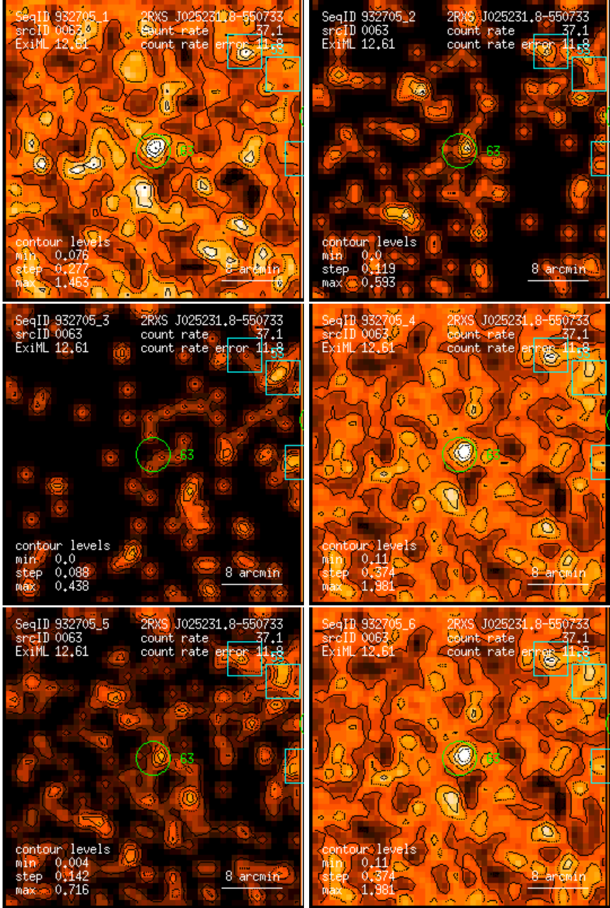
Figure 63: RASS 932705: detection 0063: band rate images, Gaussian filter: (1) PSPC channels 11 – 41, (2) 52 – 90, (3) 91 – 201, (4) 11 – 235, (5) 52 – 201, (6) 11 – 201. Broad band rates in counts/ks. Band rate contour levels in counts/ks/arcmin 2 .
