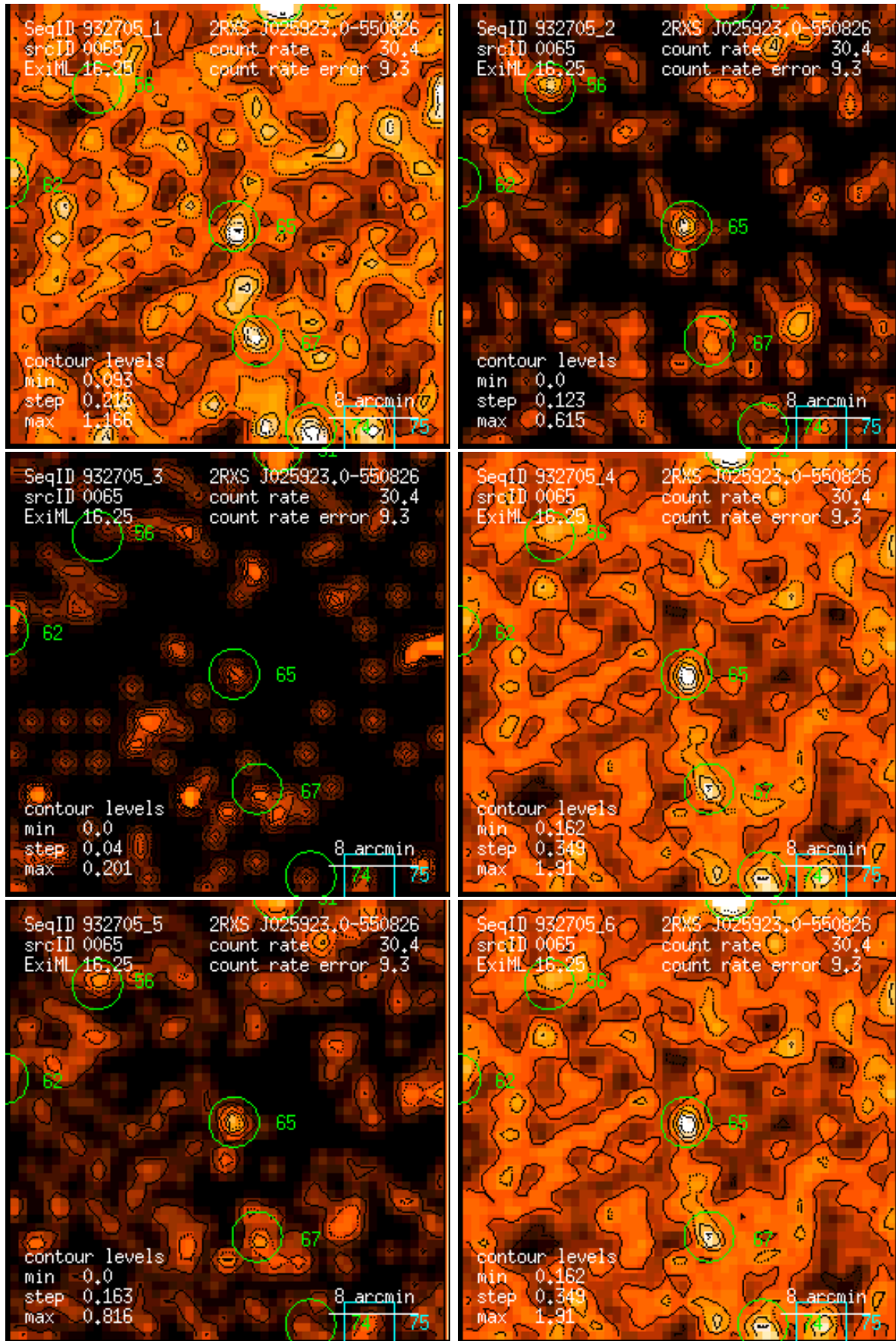
Figure 65: RASS 932705: detection 0065: band rate images, Gaussian filter: (1) PSPC channels 11 – 41, (2) 52 – 90, (3) 91 – 201, (4) 11 – 235, (5) 52 – 201, (6) 11 – 201. Broad band rates in counts/ks. Band rate contour levels in counts/ks/arcmin 2 .
