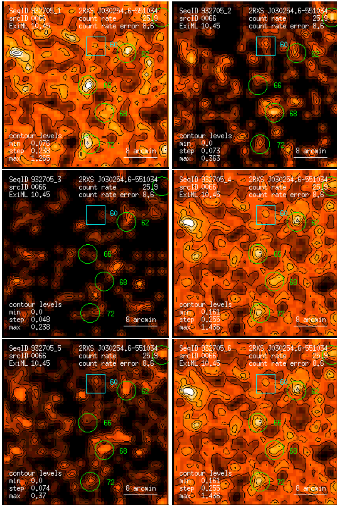
Figure 66: RASS 932705: detection 0066: band rate images, Gaussian filter: (1) PSPC channels 11 – 41, (2) 52 – 90, (3) 91 – 201, (4) 11 – 235, (5) 52 – 201, (6) 11 – 201. Broad band rates in counts/ks. Band rate contour levels in counts/ks/arcmin 2 .
