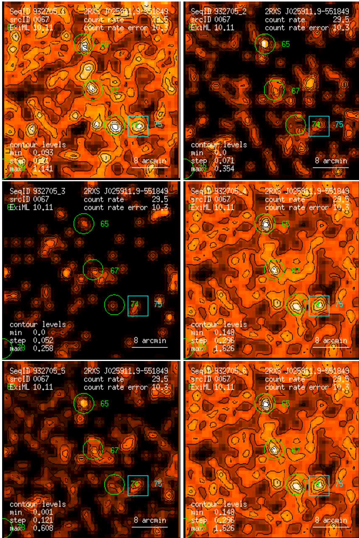
Figure 67: RASS 932705: detection 0067: band rate images, Gaussian filter: (1) PSPC channels 11 – 41, (2) 52 – 90, (3) 91 – 201, (4) 11 – 235, (5) 52 – 201, (6) 11 – 201. Broad band rates in counts/ks. Band rate contour levels in counts/ks/arcmin 2 .
