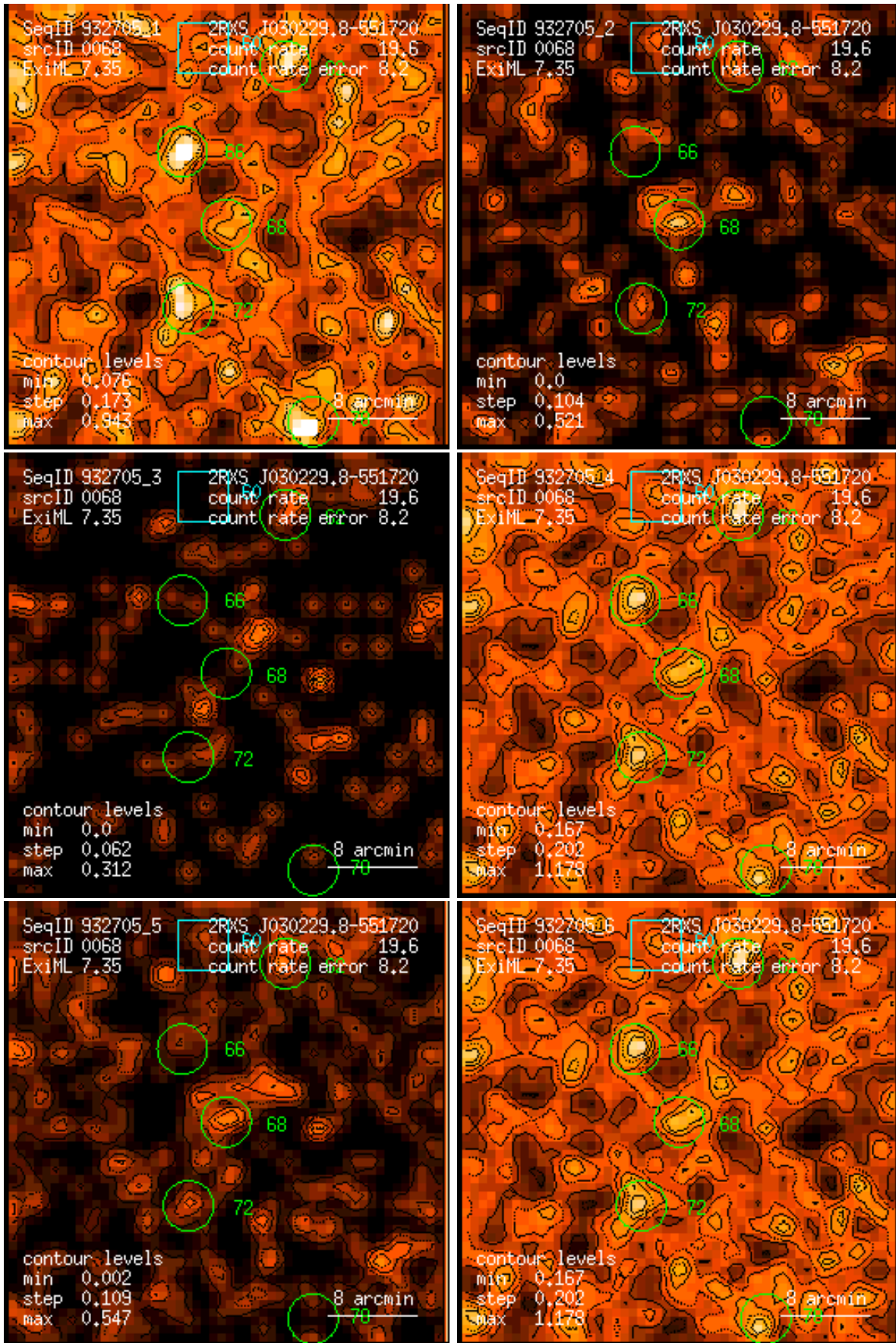
Figure 68: RASS 932705: detection 0068: band rate images, Gaussian filter: (1) PSPC channels 11 – 41, (2) 52 – 90, (3) 91 – 201, (4) 11 – 235, (5) 52 – 201, (6) 11 – 201. Broad band rates in counts/ks. Band rate contour levels in counts/ks/arcmin 2 .
