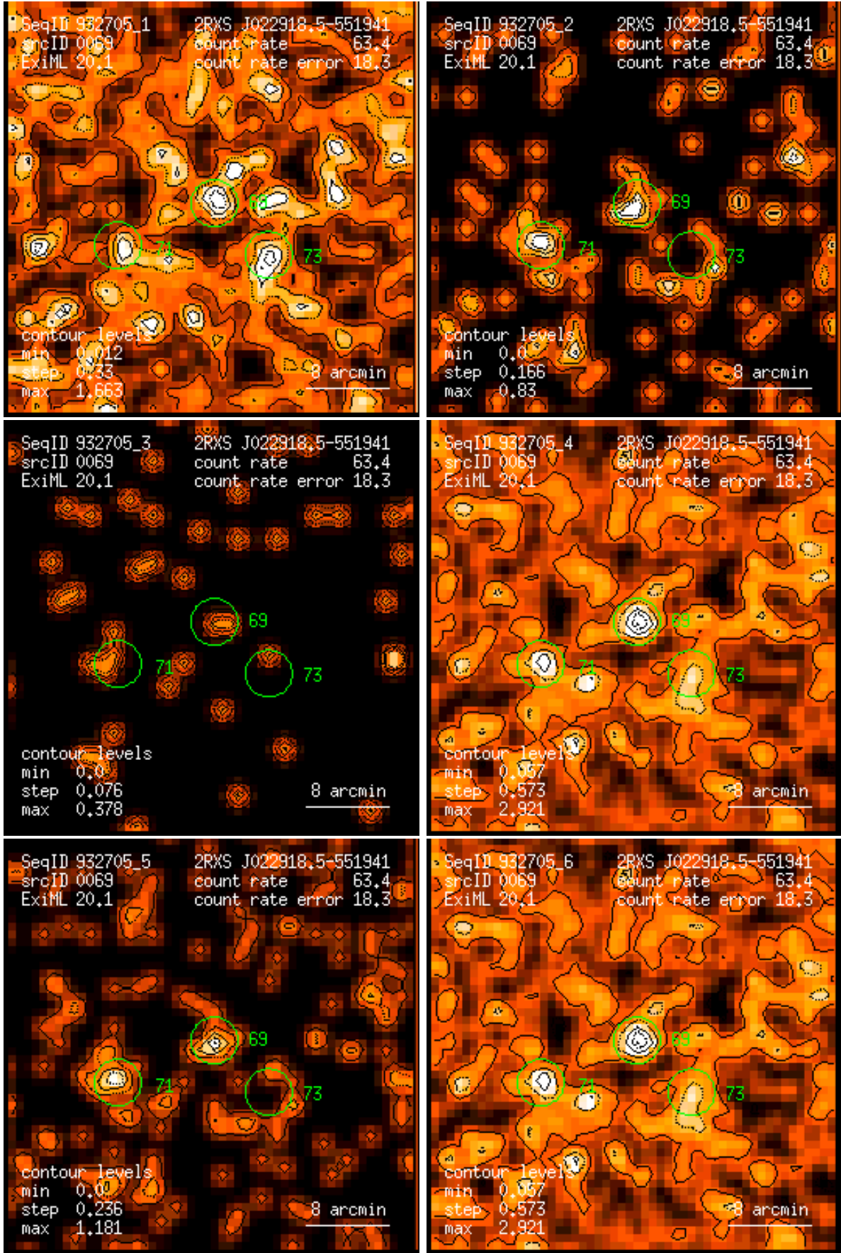
Figure 69: RASS 932705: detection 0069: band rate images, Gaussian filter: (1) PSPC channels 11 – 41, (2) 52 – 90, (3) 91 – 201, (4) 11 – 235, (5) 52 – 201, (6) 11 – 201. Broad band rates in counts/ks. Band rate contour levels in counts/ks/arcmin 2 .
