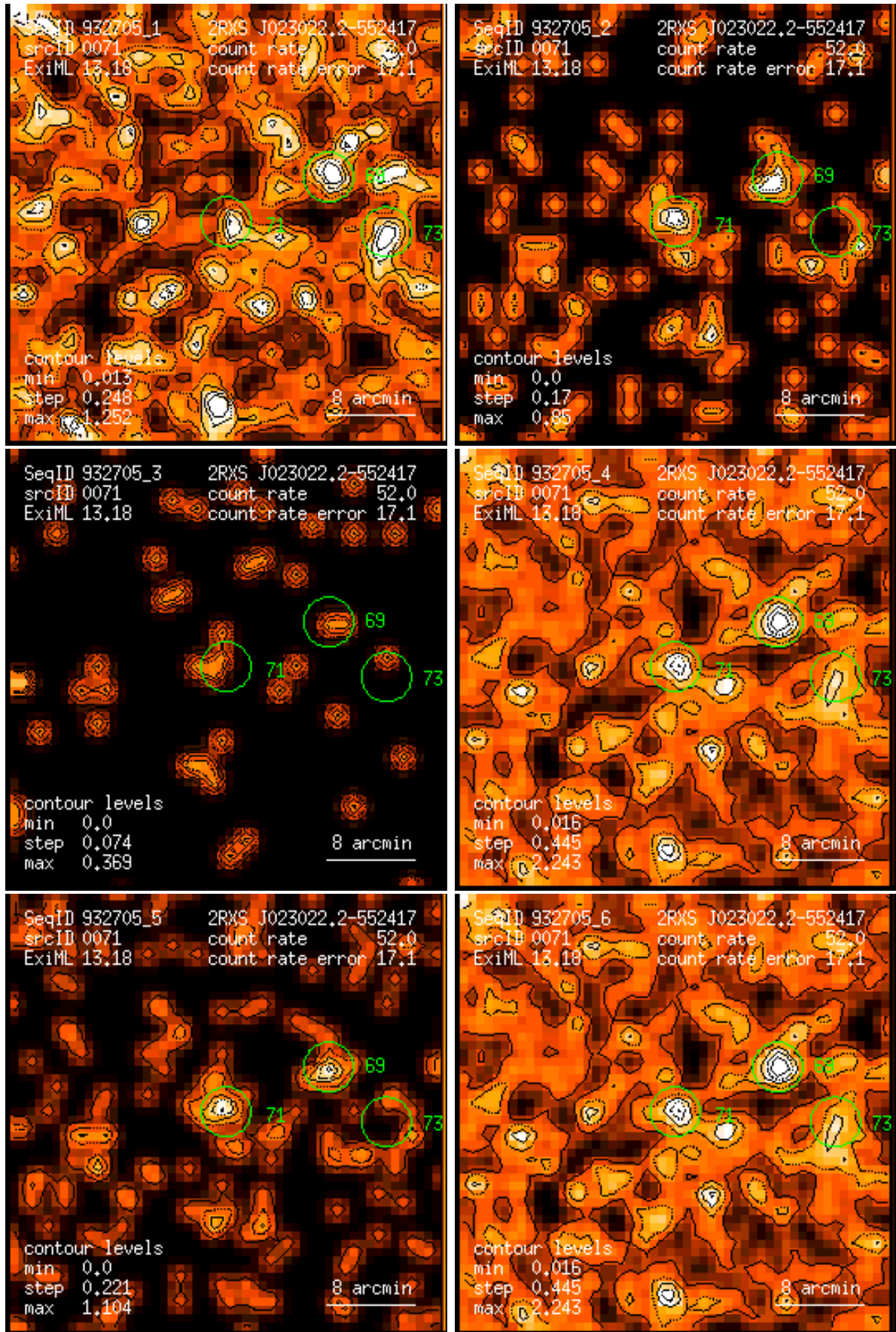
Figure 71: RASS 932705: detection 0071: band rate images, Gaussian filter: (1) PSPC channels 11 – 41, (2) 52 – 90, (3) 91 – 201, (4) 11 – 235, (5) 52 – 201, (6) 11 – 201. Broad band rates in counts/ks. Band rate contour levels in counts/ks/arcmin 2 .
