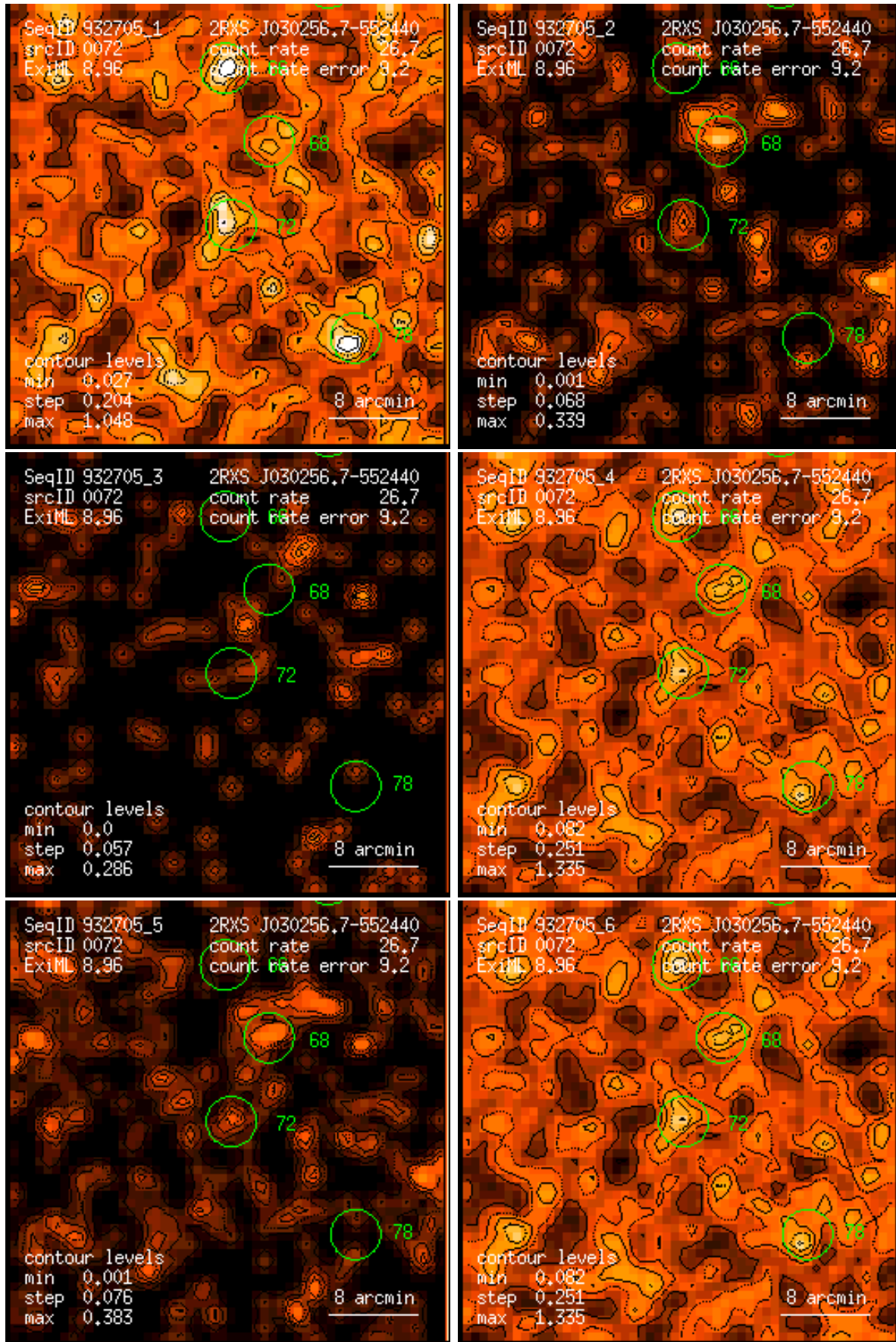
Figure 72: RASS 932705: detection 0072: band rate images, Gaussian filter: (1) PSPC channels 11 – 41, (2) 52 – 90, (3) 91 – 201, (4) 11 – 235, (5) 52 – 201, (6) 11 – 201. Broad band rates in counts/ks. Band rate contour levels in counts/ks/arcmin 2 .
