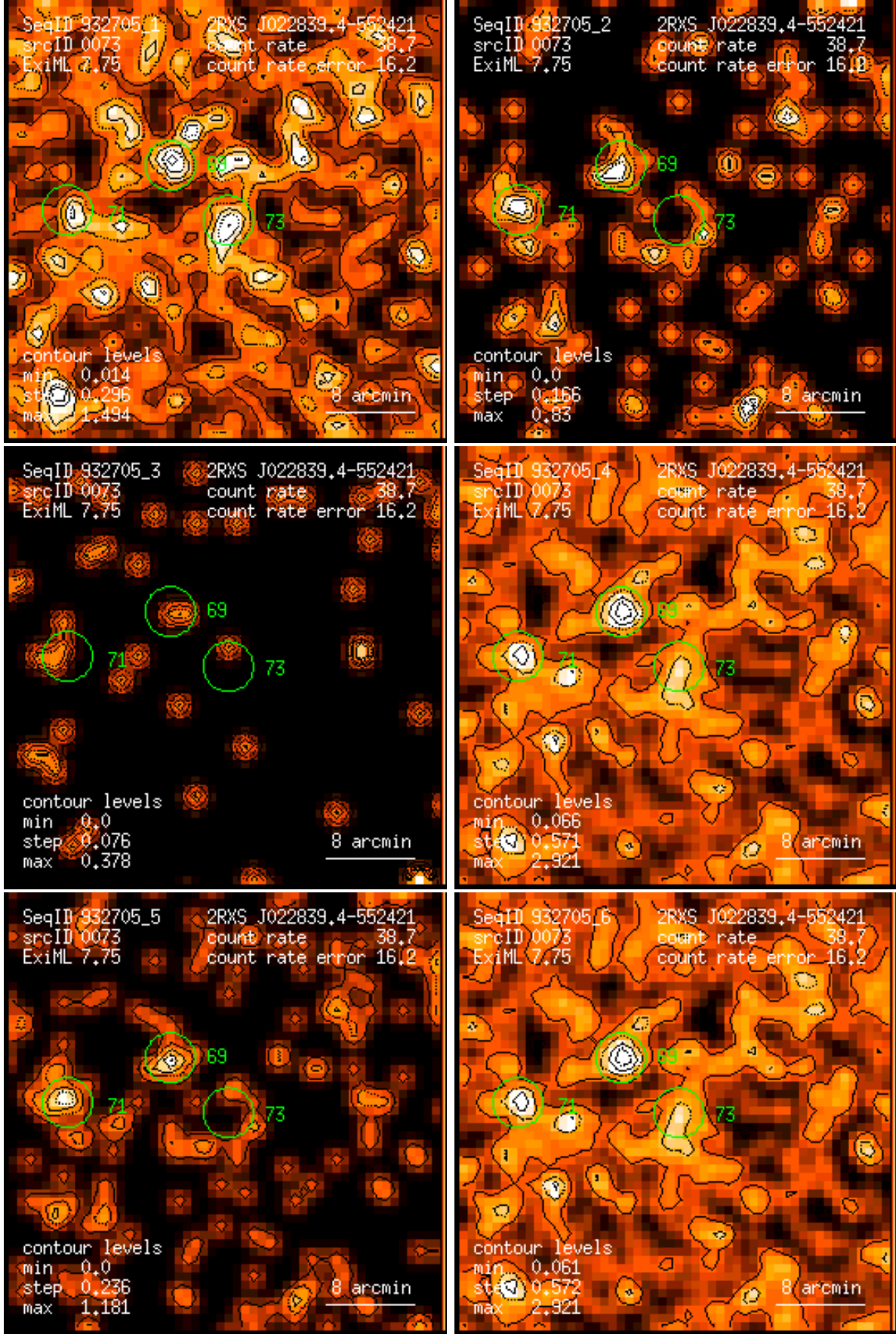
Figure 73: RASS 932705: detection 0073: band rate images, Gaussian filter: (1) PSPC channels 11 – 41, (2) 52 – 90, (3) 91 – 201, (4) 11 – 235, (5) 52 – 201, (6) 11 – 201. Broad band rates in counts/ks. Band rate contour levels in counts/ks/arcmin 2 .
