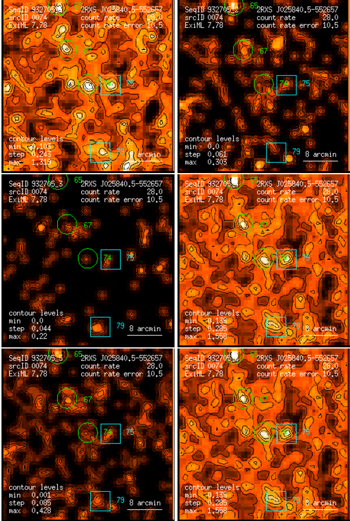
Figure 74: RASS 932705: detection 0074: band rate images, Gaussian filter: (1) PSPC channels 11 – 41, (2) 52 – 90, (3) 91 – 201, (4) 11 – 235, (5) 52 – 201, (6) 11 – 201. Broad band rates in counts/ks. Band rate contour levels in counts/ks/arcmin 2 .
