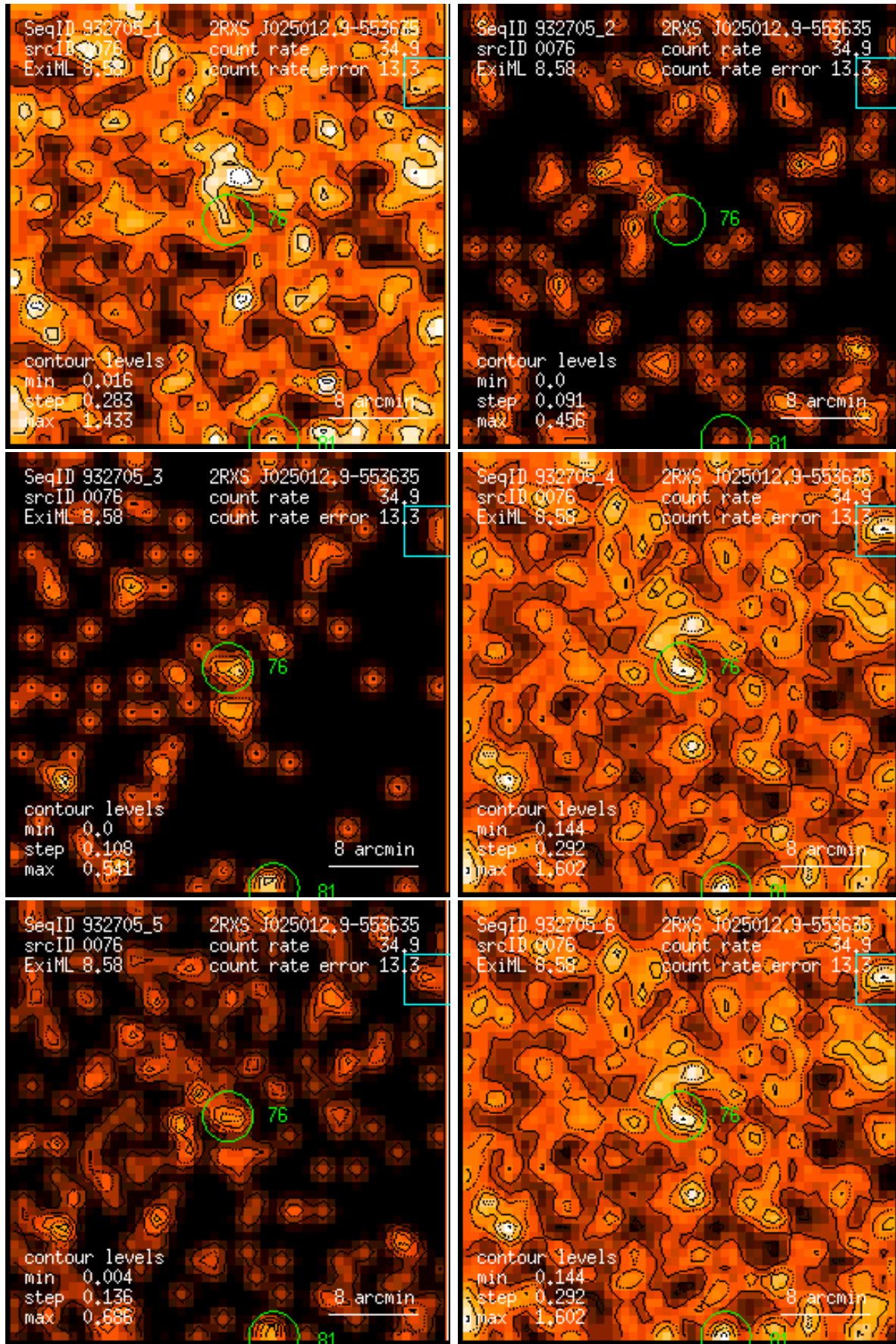
Figure 76: RASS 932705: detection 0076: band rate images, Gaussian filter: (1) PSPC channels 11 – 41, (2) 52 – 90, (3) 91 – 201, (4) 11 – 235, (5) 52 – 201, (6) 11 – 201. Broad band rates in counts/ks. Band rate contour levels in counts/ks/arcmin 2 .
