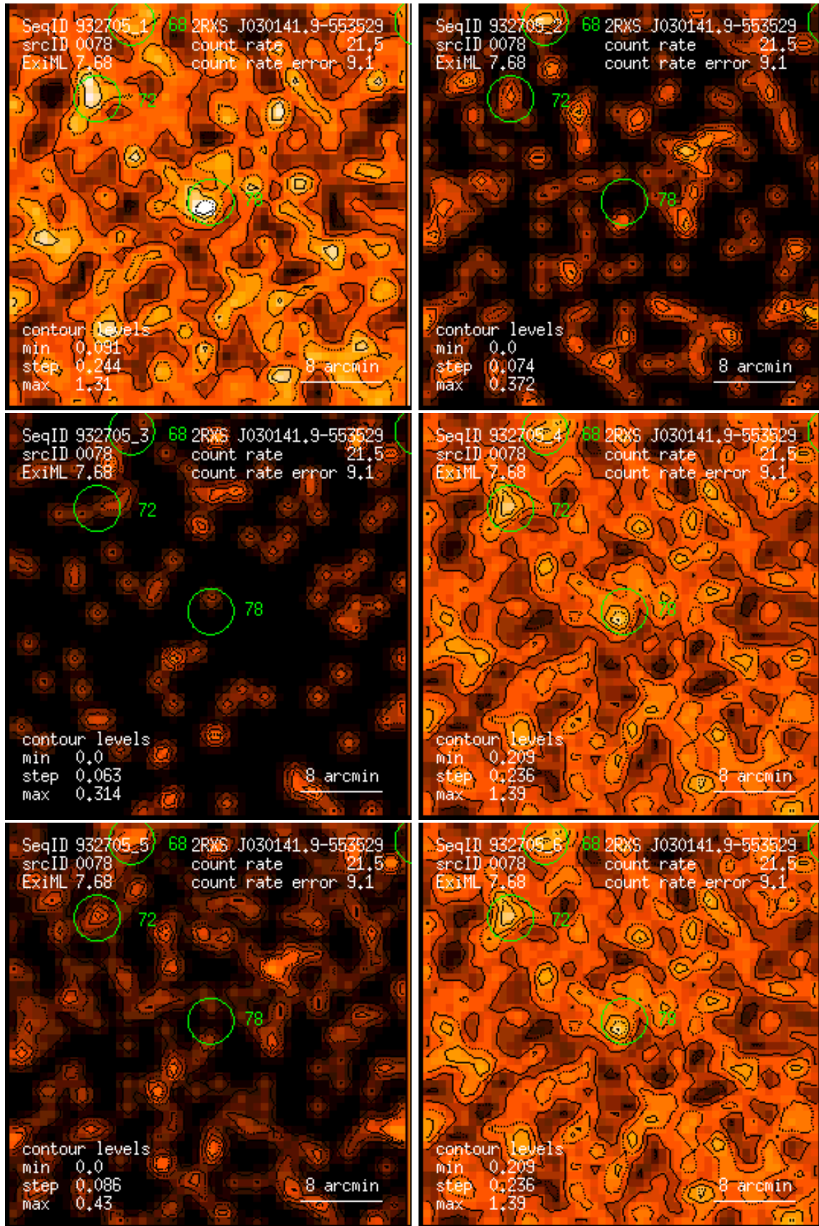
Figure 78: RASS 932705: detection 0078: band rate images, Gaussian filter: (1) PSPC channels 11 – 41, (2) 52 – 90, (3) 91 – 201, (4) 11 – 235, (5) 52 – 201, (6) 11 – 201. Broad band rates in counts/ks. Band rate contour levels in counts/ks/arcmin 2 .
