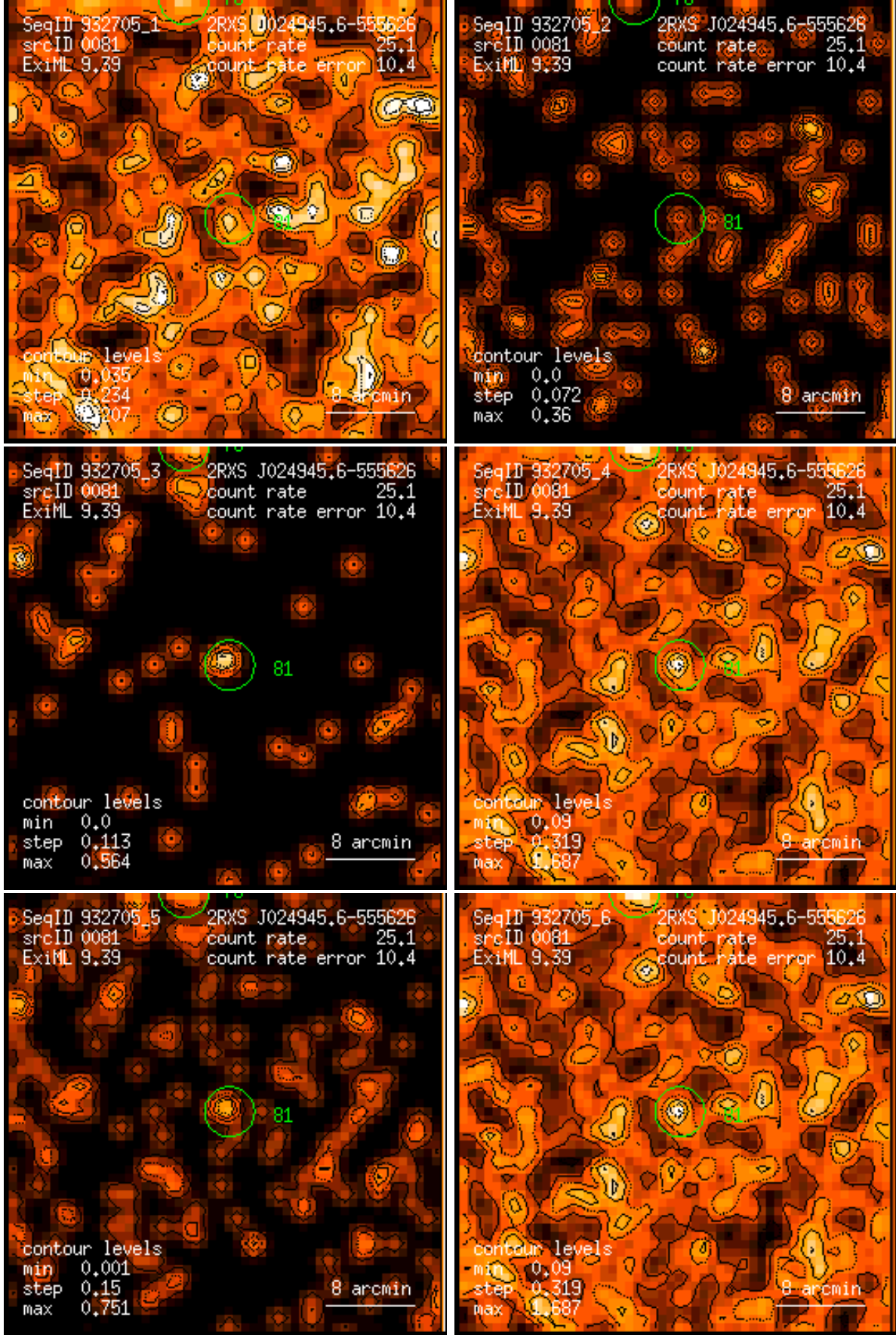
Figure 81: RASS 932705: detection 0081: band rate images, Gaussian filter: (1) PSPC channels 11 – 41, (2) 52 – 90, (3) 91 – 201, (4) 11 – 235, (5) 52 – 201, (6) 11 – 201. Broad band rates in counts/ks. Band rate contour levels in counts/ks/arcmin 2 .
