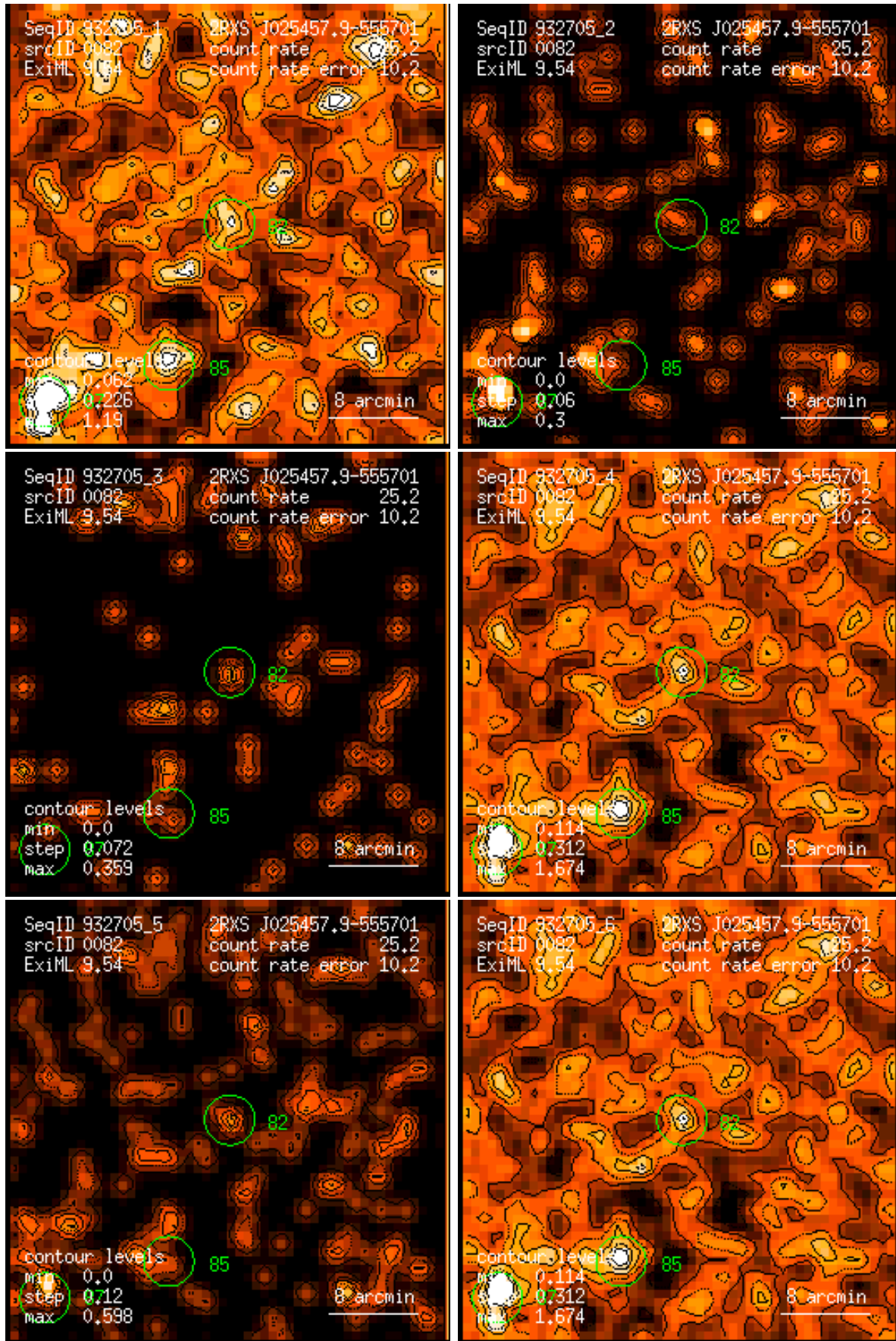
Figure 82: RASS 932705: detection 0082: band rate images, Gaussian filter: (1) PSPC channels 11 – 41, (2) 52 – 90, (3) 91 – 201, (4) 11 – 235, (5) 52 – 201, (6) 11 – 201. Broad band rates in counts/ks. Band rate contour levels in counts/ks/arcmin 2 .
