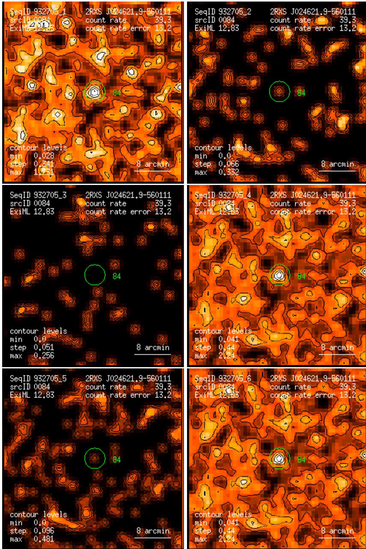
Figure 84: RASS 932705: detection 0084: band rate images, Gaussian filter: (1) PSPC channels 11 – 41, (2) 52 – 90, (3) 91 – 201, (4) 11 – 235, (5) 52 – 201, (6) 11 – 201. Broad band rates in counts/ks. Band rate contour levels in counts/ks/arcmin 2 .
