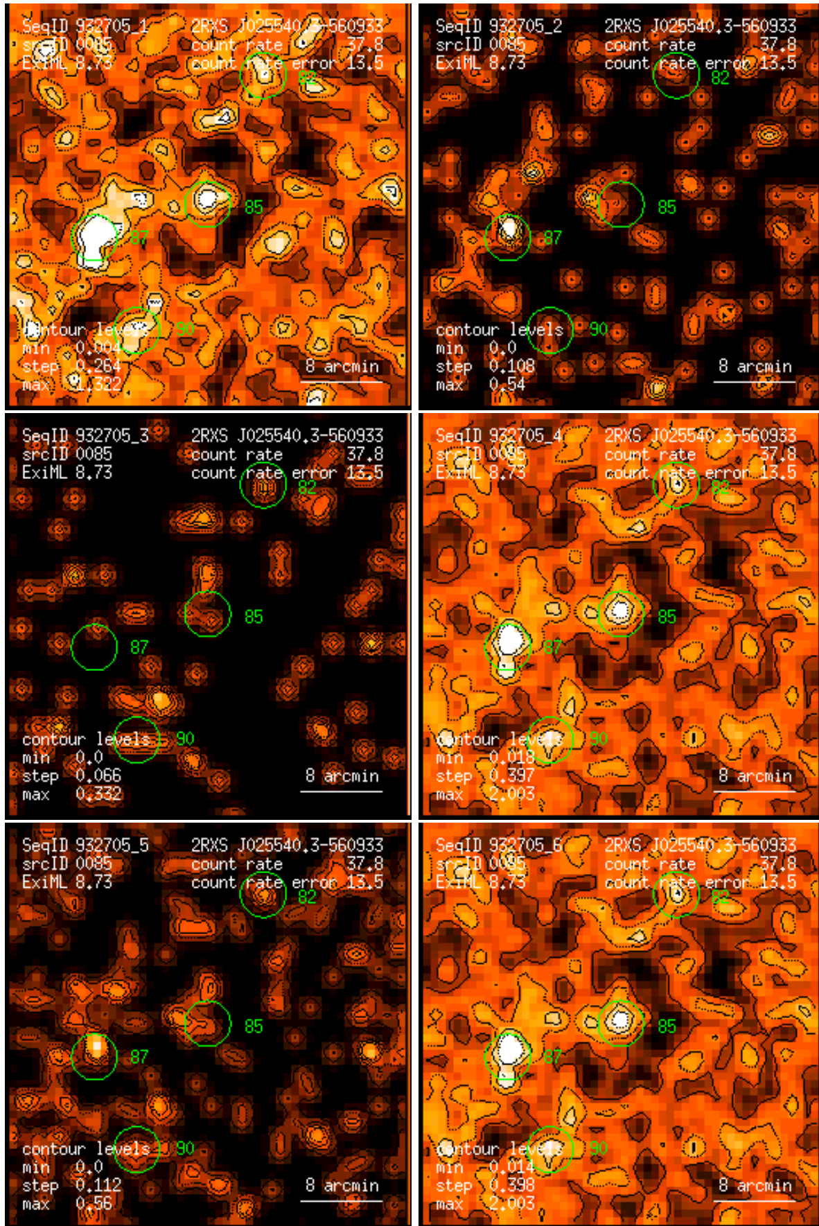
Figure 85: RASS 932705: detection 0085: band rate images, Gaussian filter: (1) PSPC channels 11 – 41, (2) 52 – 90, (3) 91 – 201, (4) 11 – 235, (5) 52 – 201, (6) 11 – 201. Broad band rates in counts/ks. Band rate contour levels in counts/ks/arcmin 2 .
