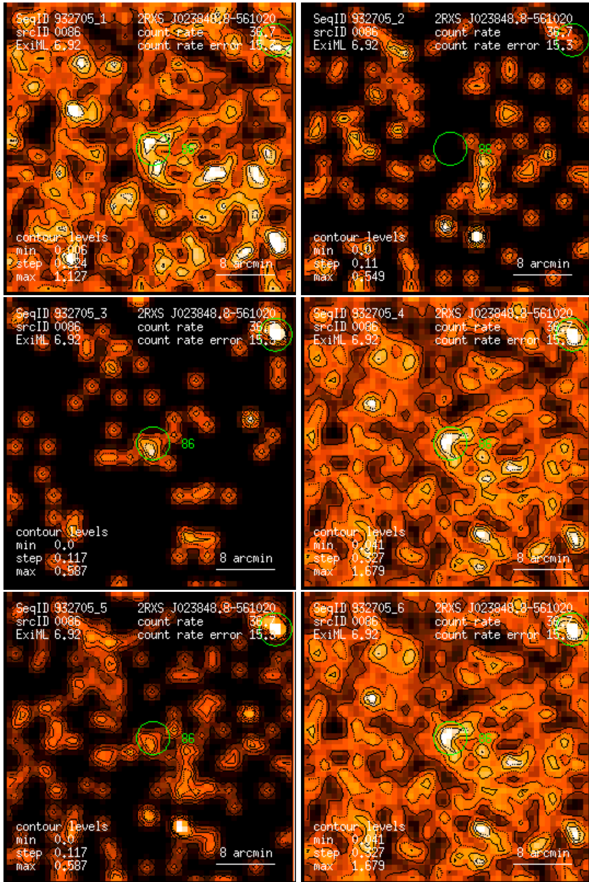
Figure 86: RASS 932705: detection 0086: band rate images, Gaussian filter: (1) PSPC channels 11 – 41, (2) 52 – 90, (3) 91 – 201, (4) 11 – 235, (5) 52 – 201, (6) 11 – 201. Broad band rates in counts/ks. Band rate contour levels in counts/ks/arcmin 2 .
