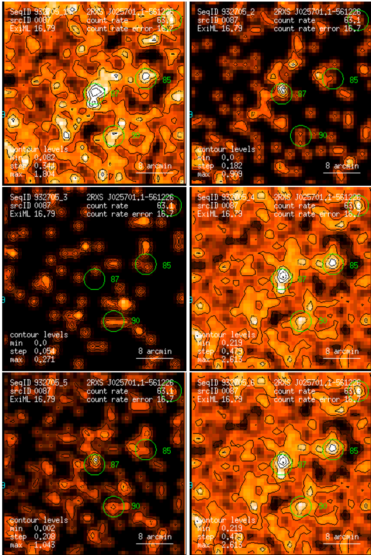
Figure 87: RASS 932705: detection 0087: band rate images, Gaussian filter: (1) PSPC channels 11 – 41, (2) 52 – 90, (3) 91 – 201, (4) 11 – 235, (5) 52 – 201, (6) 11 – 201. Broad band rates in counts/ks. Band rate contour levels in counts/ks/arcmin 2 .
