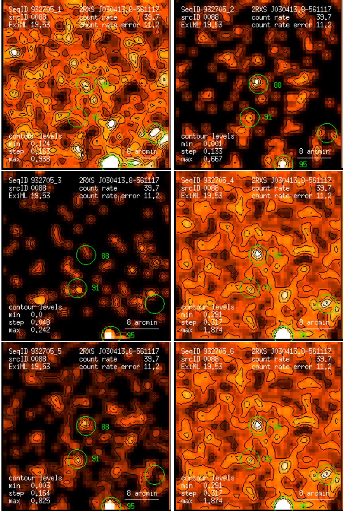
Figure 88: RASS 932705: detection 0088: band rate images, Gaussian filter: (1) PSPC channels 11 – 41, (2) 52 – 90, (3) 91 – 201, (4) 11 – 235, (5) 52 – 201, (6) 11 – 201. Broad band rates in counts/ks. Band rate contour levels in counts/ks/arcmin 2 .
