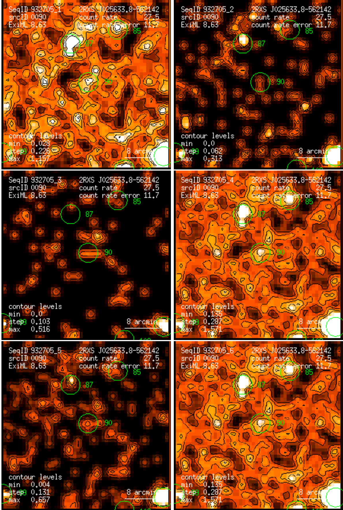
Figure 90: RASS 932705: detection 0090: band rate images, Gaussian filter: (1) PSPC channels 11 – 41, (2) 52 – 90, (3) 91 – 201, (4) 11 – 235, (5) 52 – 201, (6) 11 – 201. Broad band rates in counts/ks. Band rate contour levels in counts/ks/arcmin 2 .
