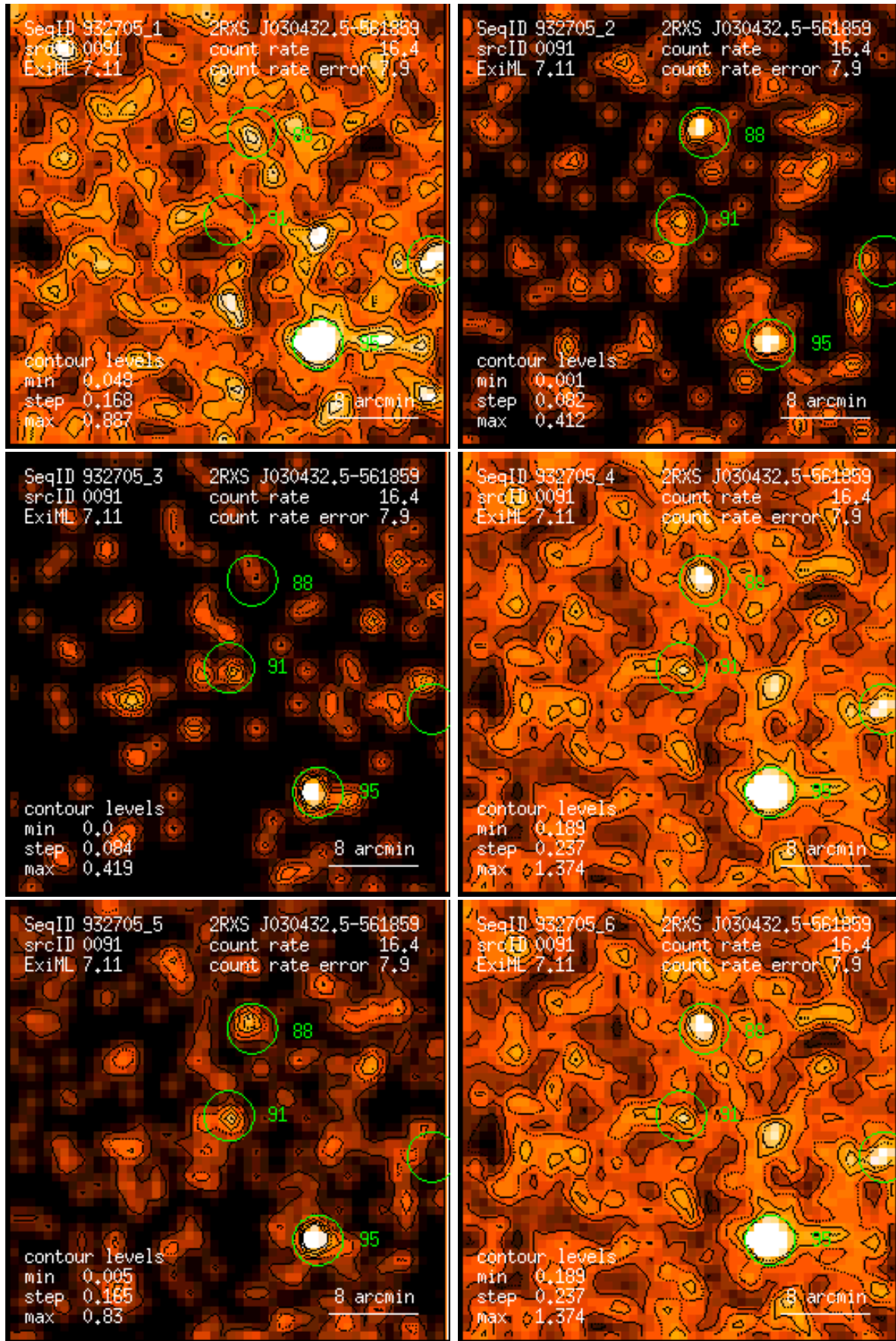
Figure 91: RASS 932705: detection 0091: band rate images, Gaussian filter: (1) PSPC channels 11 – 41, (2) 52 – 90, (3) 91 – 201, (4) 11 – 235, (5) 52 – 201, (6) 11 – 201. Broad band rates in counts/ks. Band rate contour levels in counts/ks/arcmin 2 .
