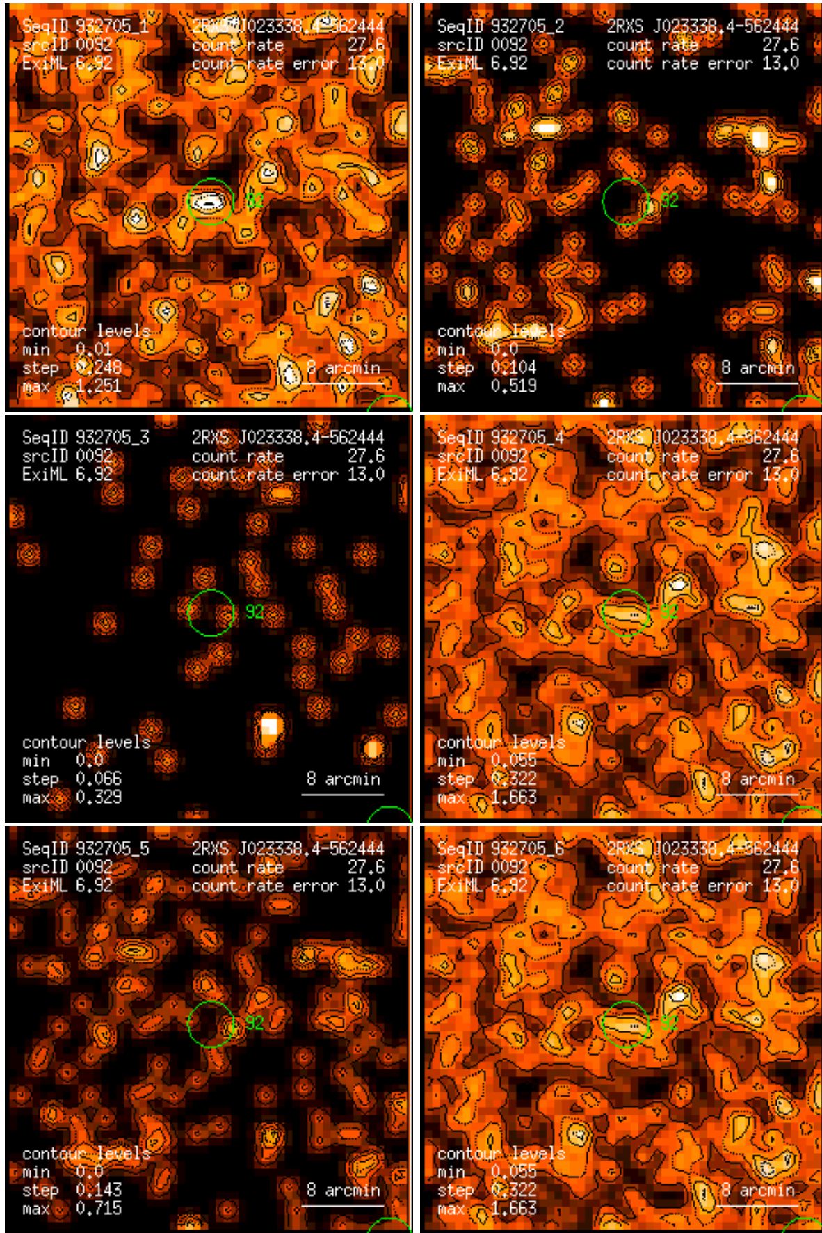
Figure 92: RASS 932705: detection 0092: band rate images, Gaussian filter: (1) PSPC channels 11 – 41, (2) 52 – 90, (3) 91 – 201, (4) 11 – 235, (5) 52 – 201, (6) 11 – 201. Broad band rates in counts/ks. Band rate contour levels in counts/ks/arcmin 2 .
