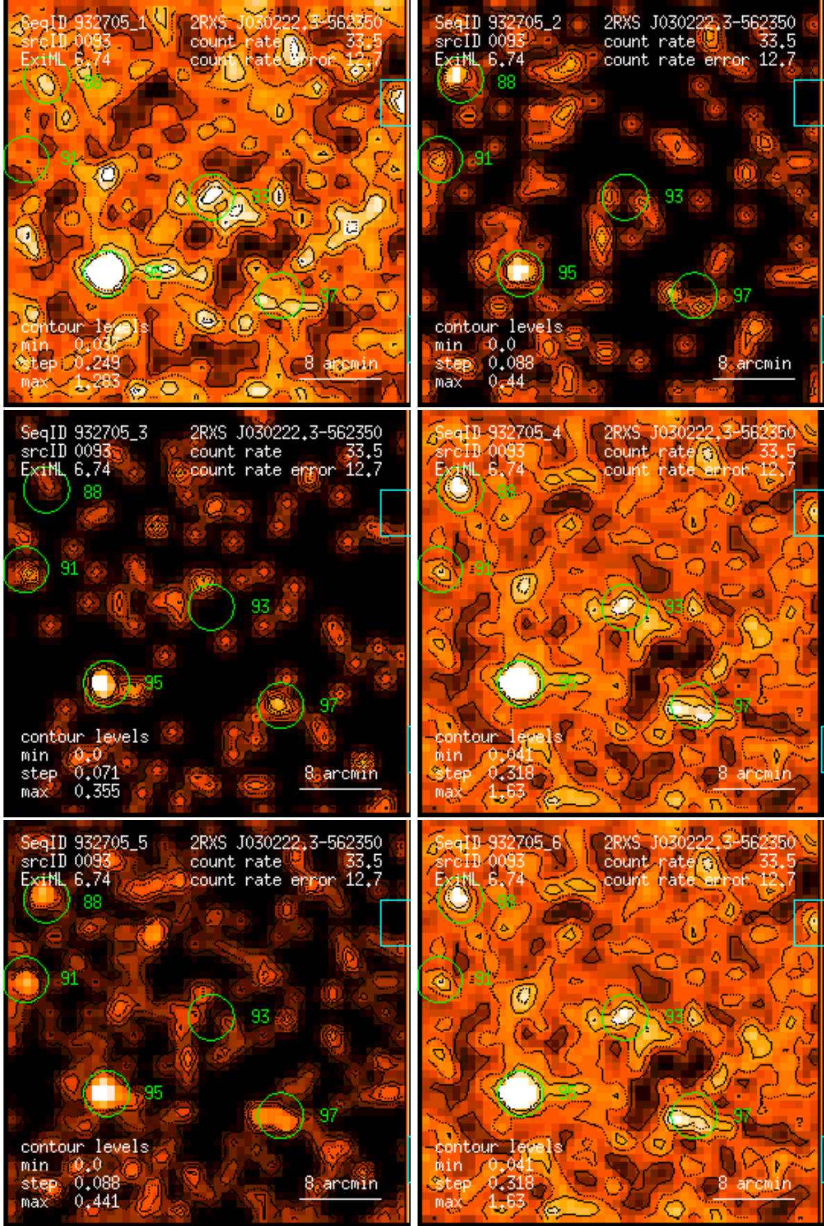
Figure 93: RASS 932705: detection 0093: band rate images, Gaussian filter: (1) PSPC channels 11 – 41, (2) 52 – 90, (3) 91 – 201, (4) 11 – 235, (5) 52 – 201, (6) 11 – 201. Broad band rates in counts/ks. Band rate contour levels in counts/ks/arcmin 2 .
