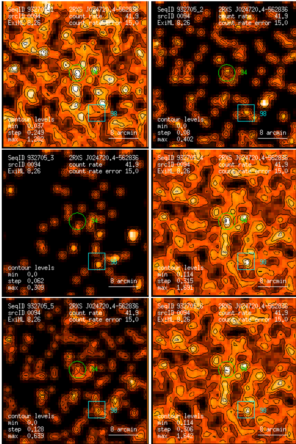
Figure 94: RASS 932705: detection 0094: band rate images, Gaussian filter: (1) PSPC channels 11 – 41, (2) 52 – 90, (3) 91 – 201, (4) 11 – 235, (5) 52 – 201, (6) 11 – 201. Broad band rates in counts/ks. Band rate contour levels in counts/ks/arcmin 2 .
