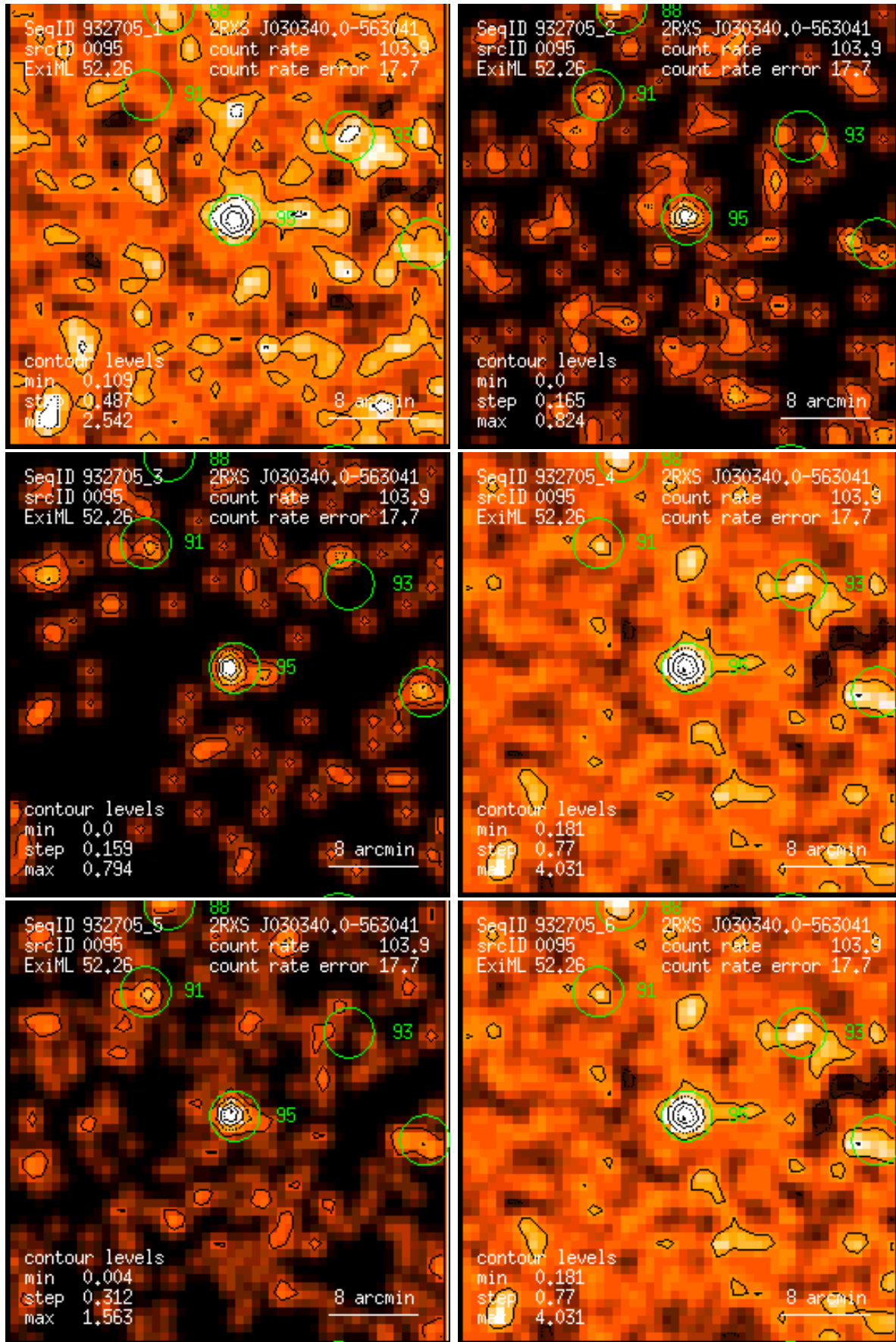
Figure 95: RASS 932705: detection 0095: band rate images, Gaussian filter: (1) PSPC channels 11 – 41, (2) 52 – 90, (3) 91 – 201, (4) 11 – 235, (5) 52 – 201, (6) 11 – 201. Broad band rates in counts/ks. Band rate contour levels in counts/ks/arcmin 2 .
