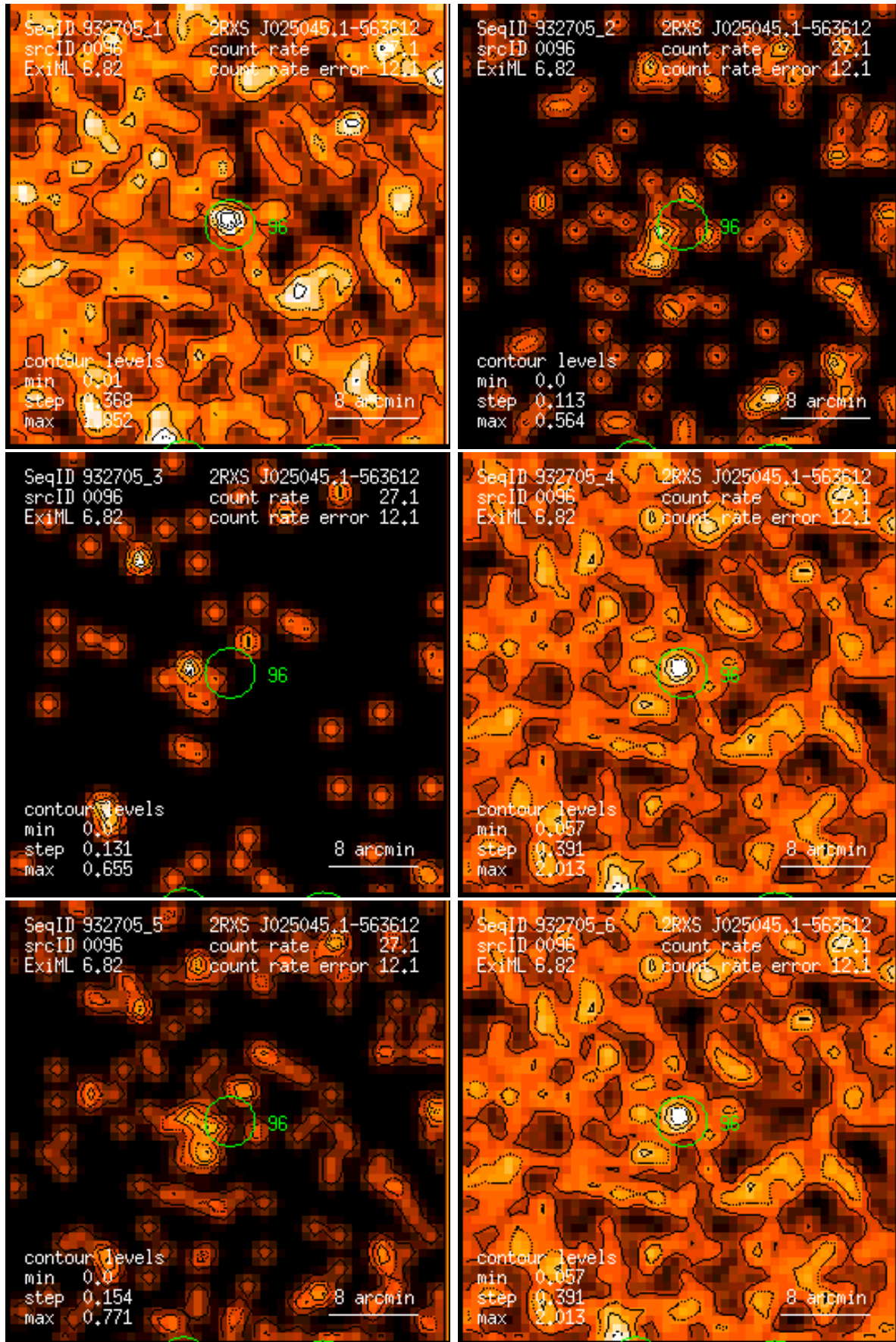
Figure 96: RASS 932705: detection 0096: band rate images, Gaussian filter: (1) PSPC channels 11 – 41, (2) 52 – 90, (3) 91 – 201, (4) 11 – 235, (5) 52 – 201, (6) 11 – 201. Broad band rates in counts/ks. Band rate contour levels in counts/ks/arcmin 2 .
