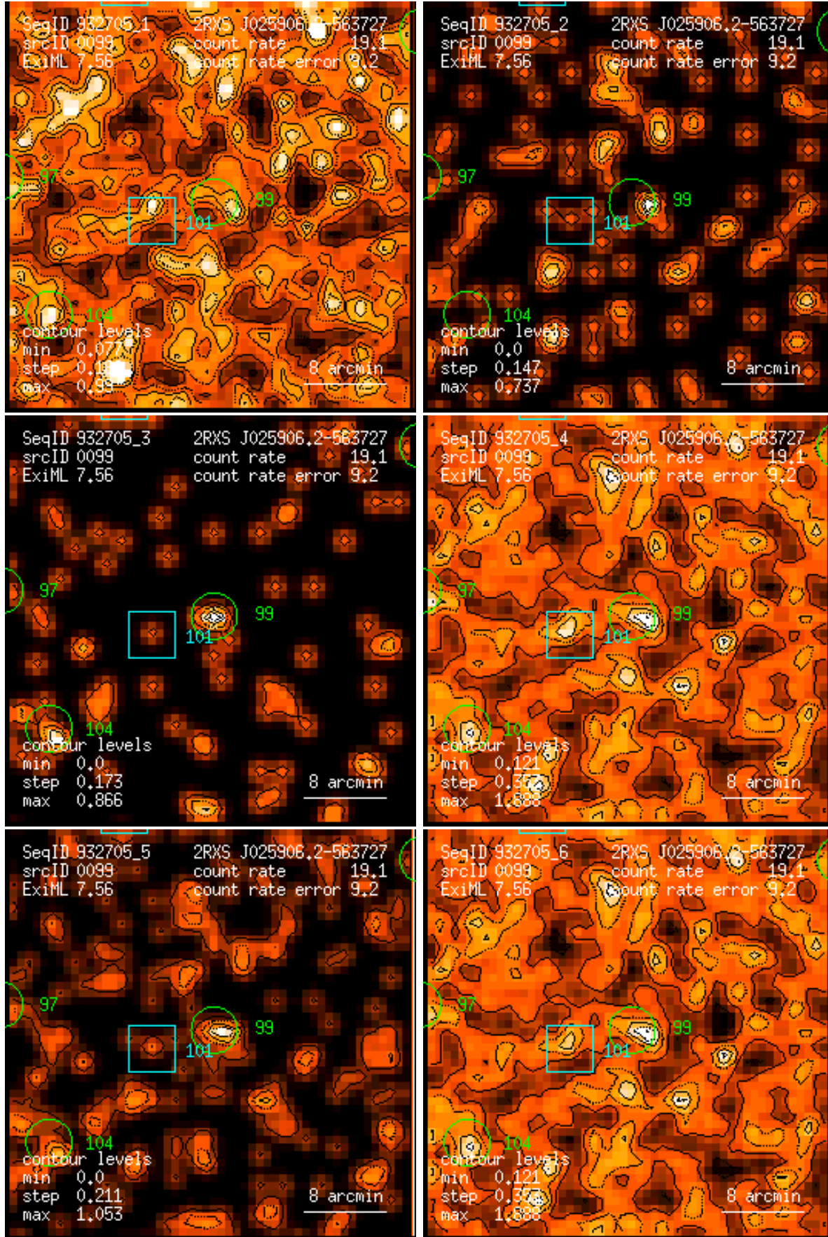
Figure 99: RASS 932705: detection 0099: band rate images, Gaussian filter: (1) PSPC channels 11 – 41, (2) 52 – 90, (3) 91 – 201, (4) 11 – 235, (5) 52 – 201, (6) 11 – 201. Broad band rates in counts/ks. Band rate contour levels in counts/ks/arcmin 2 .
