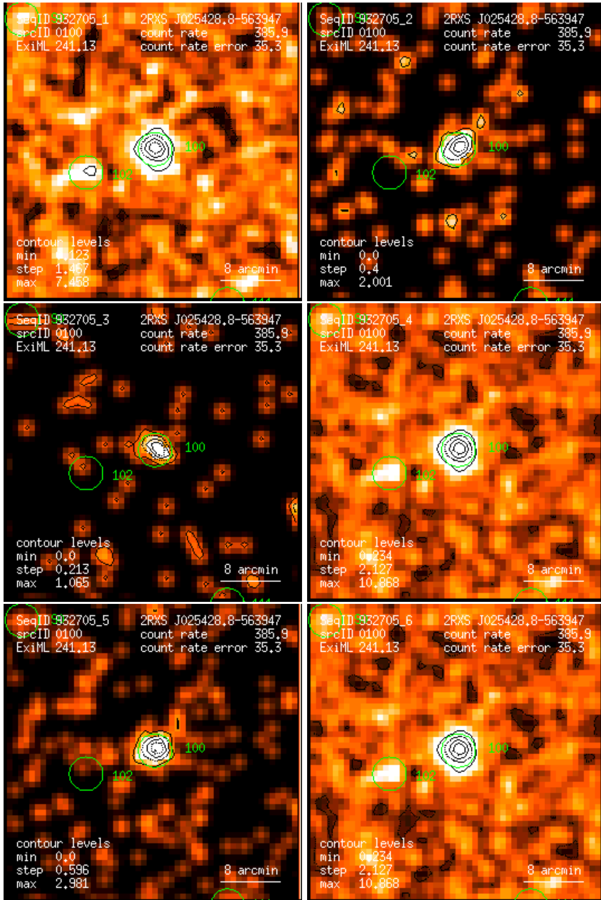
Figure 100: RASS 932705: detection 0100: band rate images, Gaussian filter: (1) PSPC channels 11 – 41, (2) 52 – 90, (3) 91 – 201, (4) 11 – 235, (5) 52 – 201, (6) 11 – 201. Broad band rates in counts/ks. Band rate contour levels in counts/ks/arcmin 2 .
