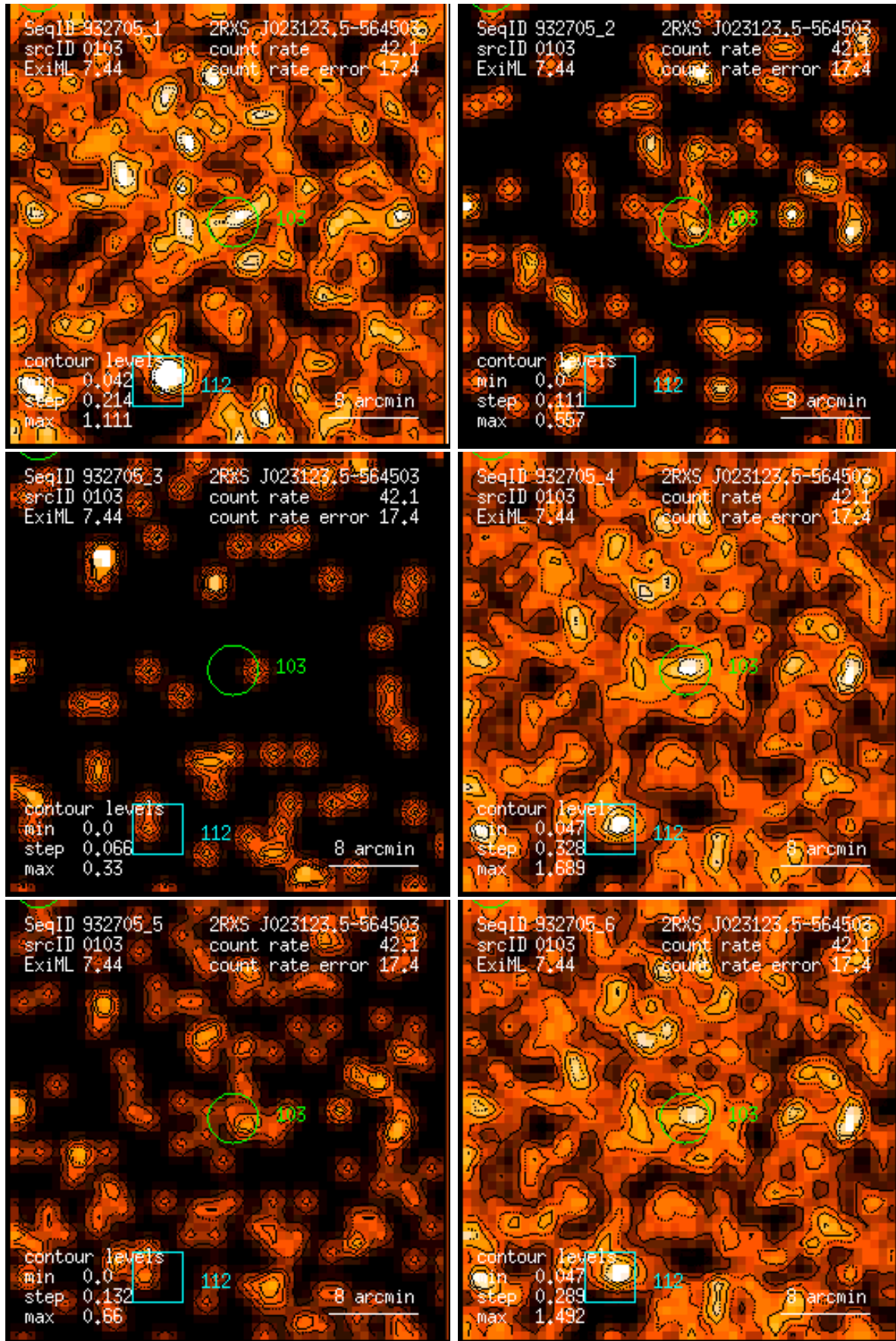
Figure 103: RASS 932705: detection 0103: band rate images, Gaussian filter: (1) PSPC channels 11 – 41, (2) 52 – 90, (3) 91 – 201, (4) 11 – 235, (5) 52 – 201, (6) 11 – 201. Broad band rates in counts/ks. Band rate contour levels in counts/ks/arcmin 2 .
