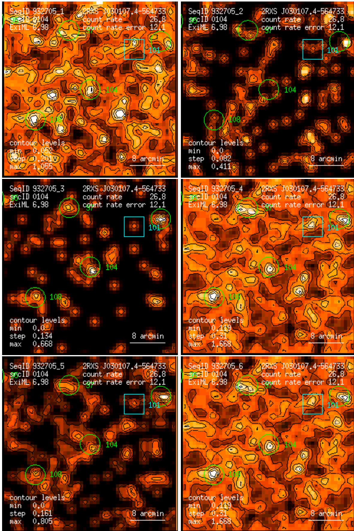
Figure 104: RASS 932705: detection 0104: band rate images, Gaussian filter: (1) PSPC channels 11 – 41, (2) 52 – 90, (3) 91 – 201, (4) 11 – 235, (5) 52 – 201, (6) 11 – 201. Broad band rates in counts/ks. Band rate contour levels in counts/ks/arcmin 2 .
