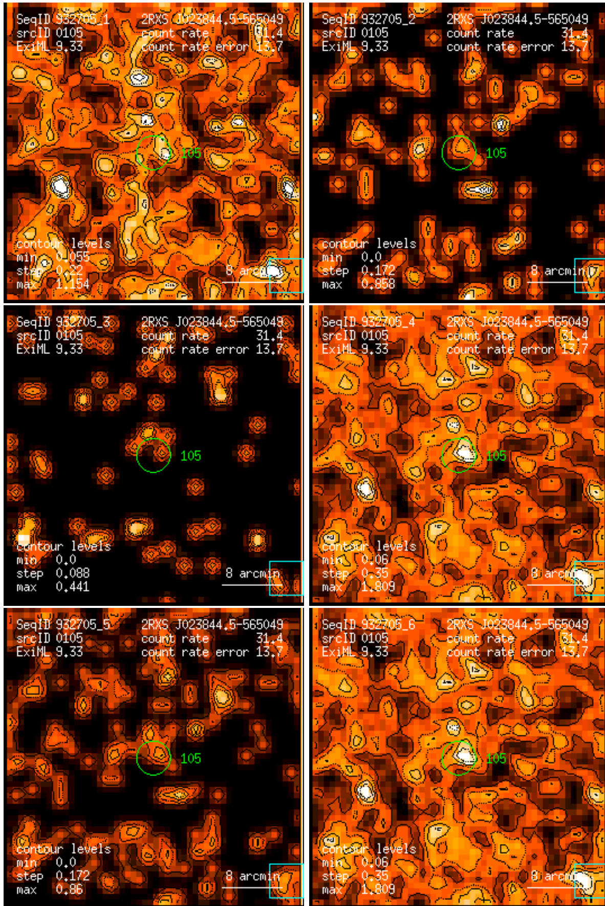
Figure 105: RASS 932705: detection 0105: band rate images, Gaussian filter: (1) PSPC channels 11 – 41, (2) 52 – 90, (3) 91 – 201, (4) 11 – 235, (5) 52 – 201, (6) 11 – 201. Broad band rates in counts/ks. Band rate contour levels in counts/ks/arcmin 2 .
